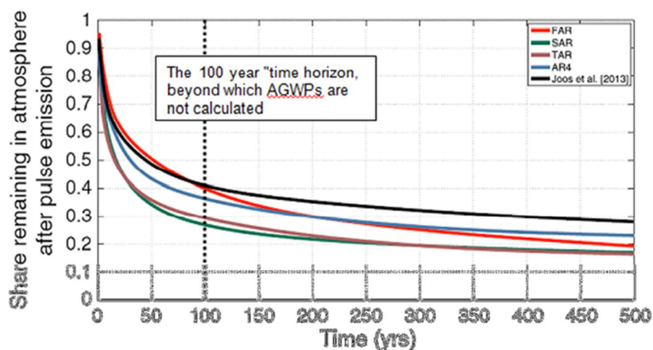
Chart: The decays in atmospheric concentration of a pulse emission of carbon dioxide used for the First, Second, Third and Fourth Assessment Reports (FAR, SAR, TAR and AR4, respectively) and the values from Joos et al. 2013 [1]
