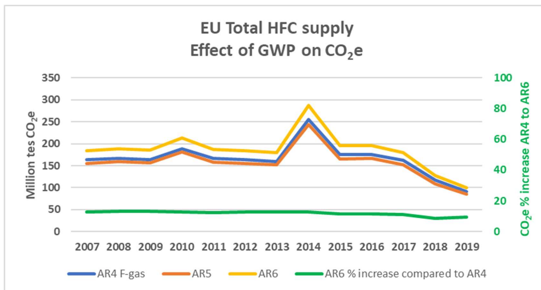
Chart- EU Reported Total Supply of HFCs, Effect of GWP on CO 2 e
