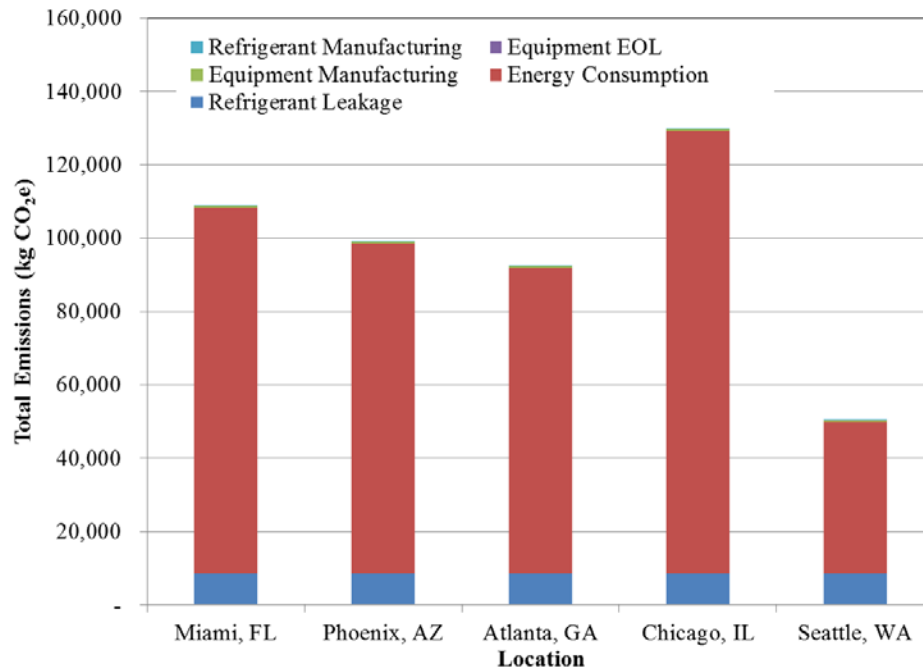
Fig. 1: LCCP Comparison for Residential Heat Pump Sample
