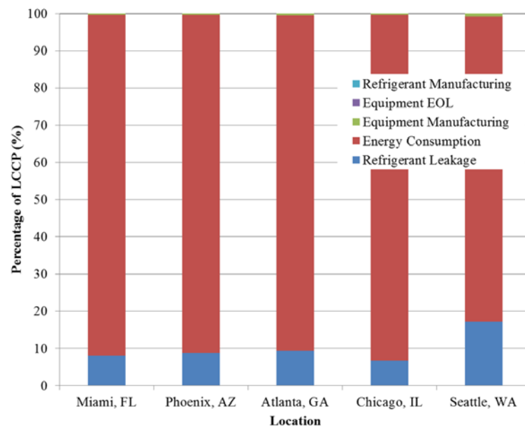
Fig 2: Composition of LCCP Percentage of Total Emissions for Residential Heat Pump Sample Problem
