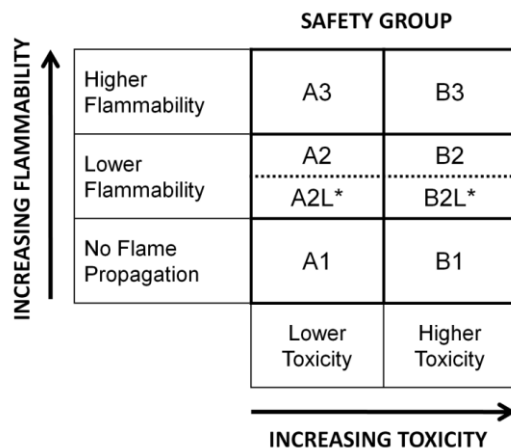
Figure 3.1: Refrigerant safety groupings in ASHRAE Standard 34-2013
