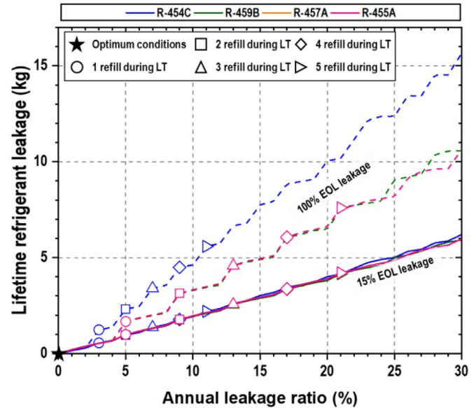
Fig. 7. Refrigerant leakage during lifetime vs. ALR.
