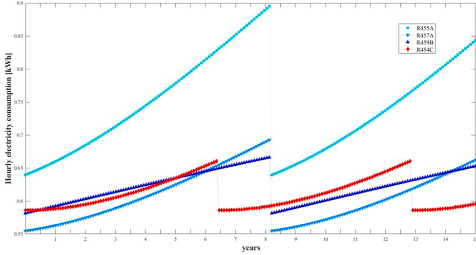
Fig. 7. Hourly electricity consumption of stand-alone.
