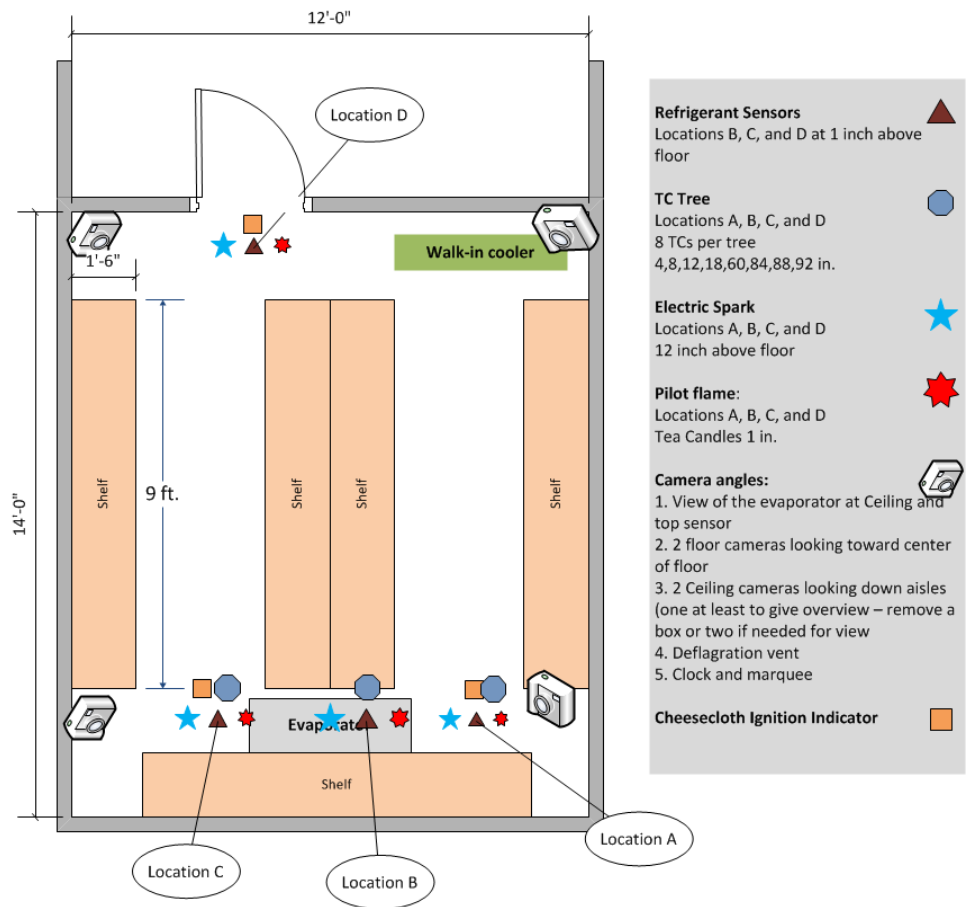
Figure 125 – Larger view of Walk-in cooler detail
