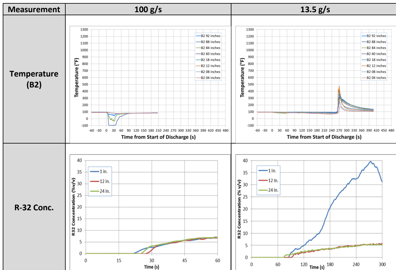
Figure 37 - Influence of Refrigerant Release Rate (100 g/s and 13.5 g/s from 2.2 m height through a 25 mm diameter opening)
