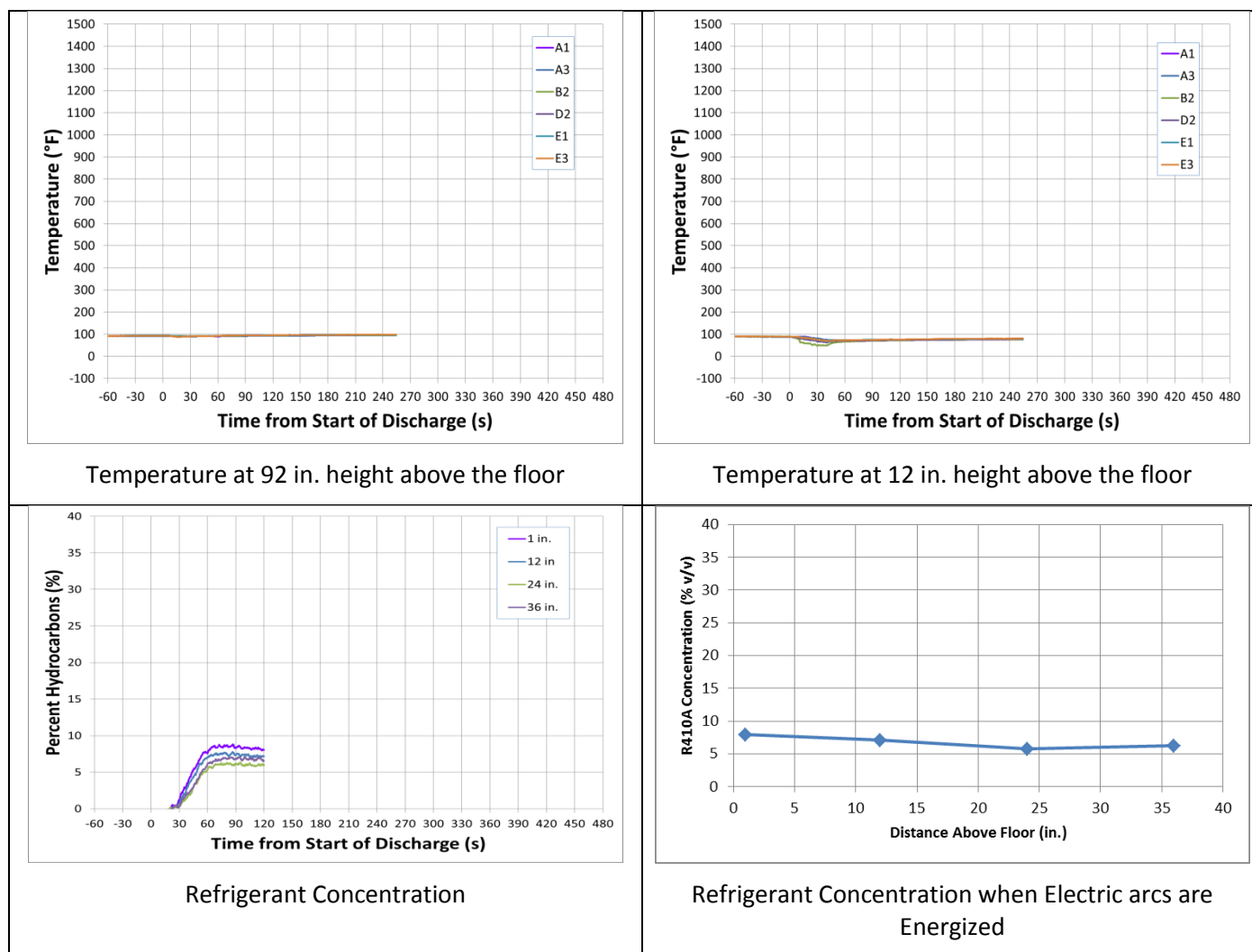
Figure 77 – Data for PC08
