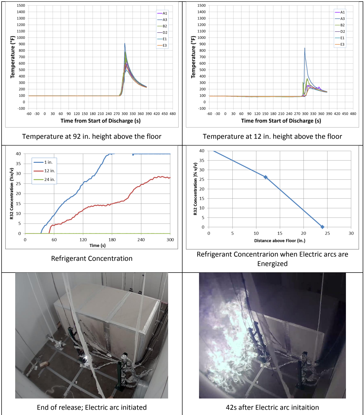
Figure 43 – Data from Cal07
