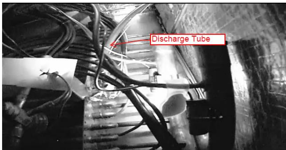
Figure 116 – Video camera view showing discharge tube near return bends
