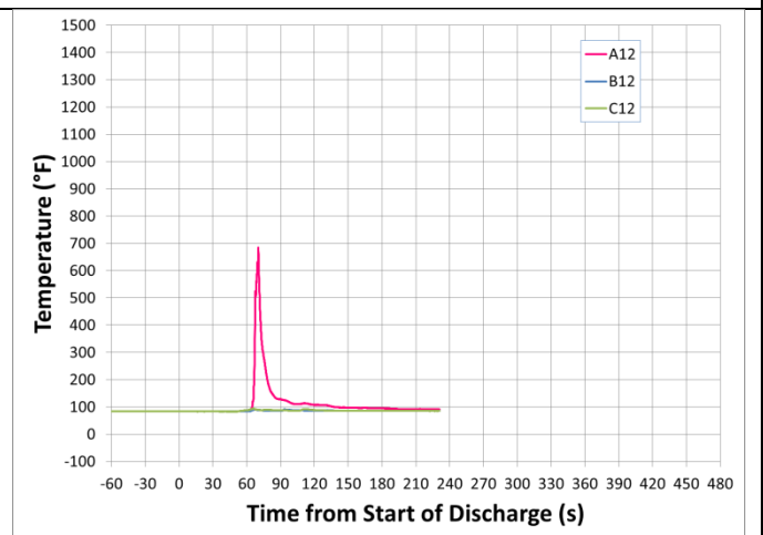
Highest temperature: Temperature 12 in. height above the floor
