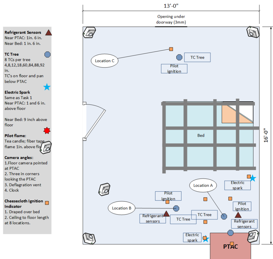
Figure 88 – Motel Room Configuration for tests PTAC11, PTAC12, and MPTAC01
