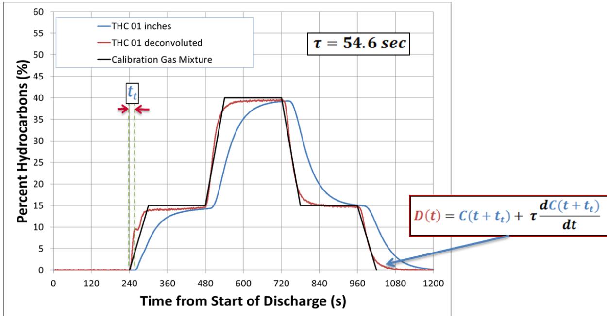
Figure 27 – Deconvolution test at 0%, 15%, and 40% concentrations
