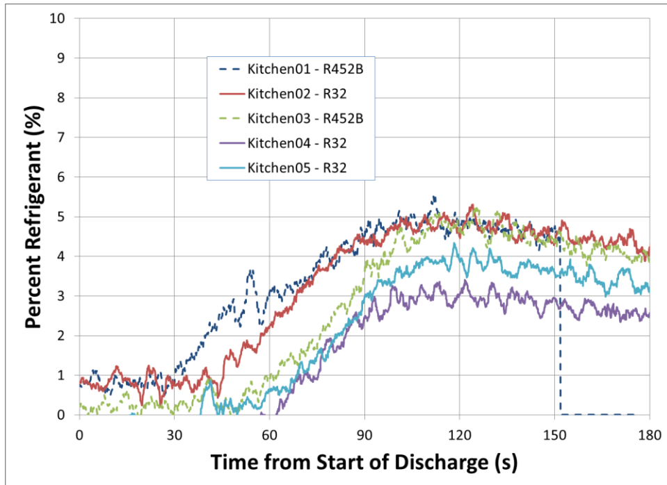
Figure 117 – Refrigerant Concentration Location B (1 inch above the floor)
