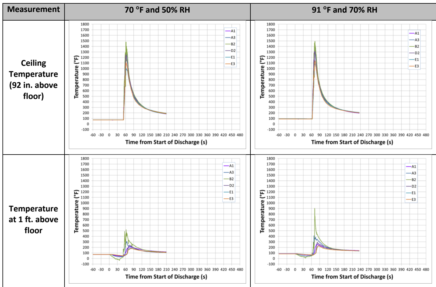
Figure 54 – Influence of Ambient Temperature and Humidity for R-32 Refrigerant
