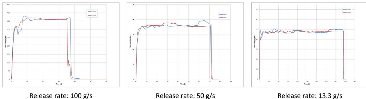
Figure 24 – Mass Flow Controller Response Time
