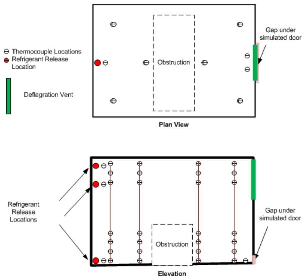
Figure 13 – Thermocouple Locations Relative to Refrigerant Release
