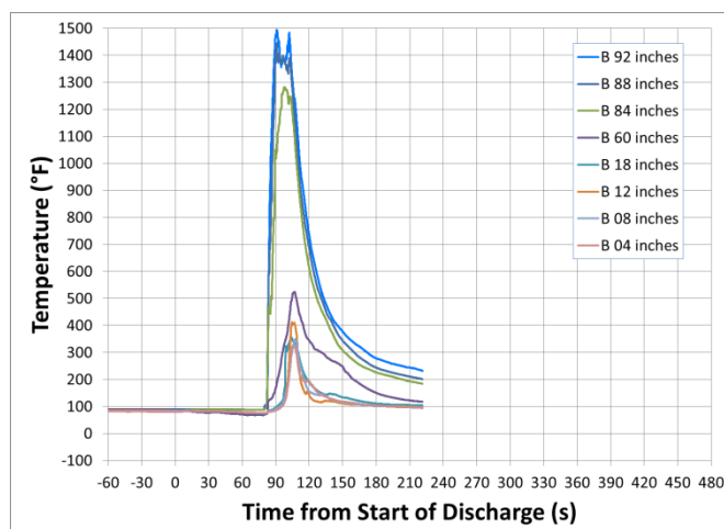
Temperature at Location B
