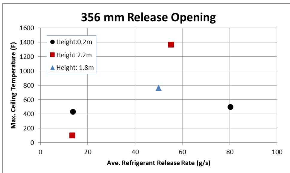
Figure 39 - Maximum Temperature Refrigerant Released from 356 mm diameter opening
