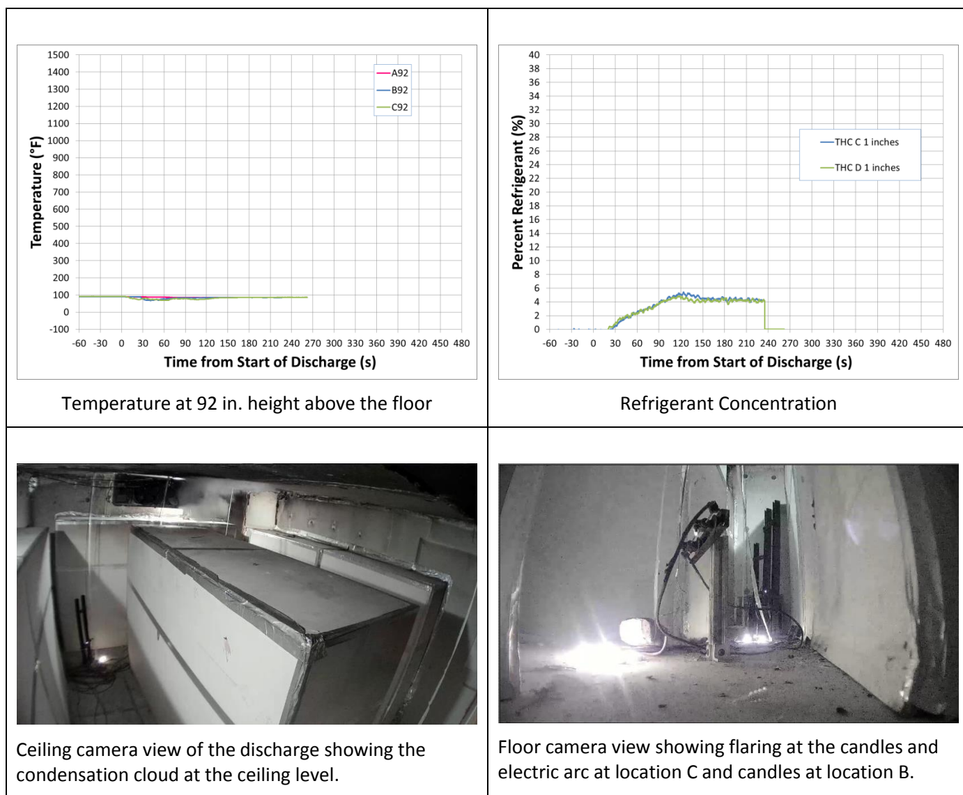
Figure 134 – Data from WALKIN14
