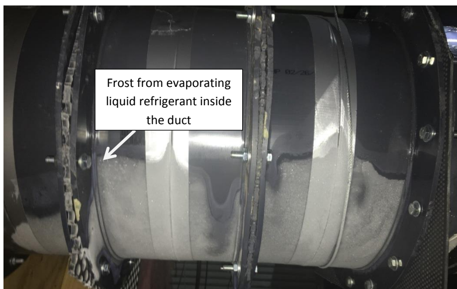
Figure 38 - Frost on the 356 mm Duct Indicating Presence of Residual Refrigerant in Duct
