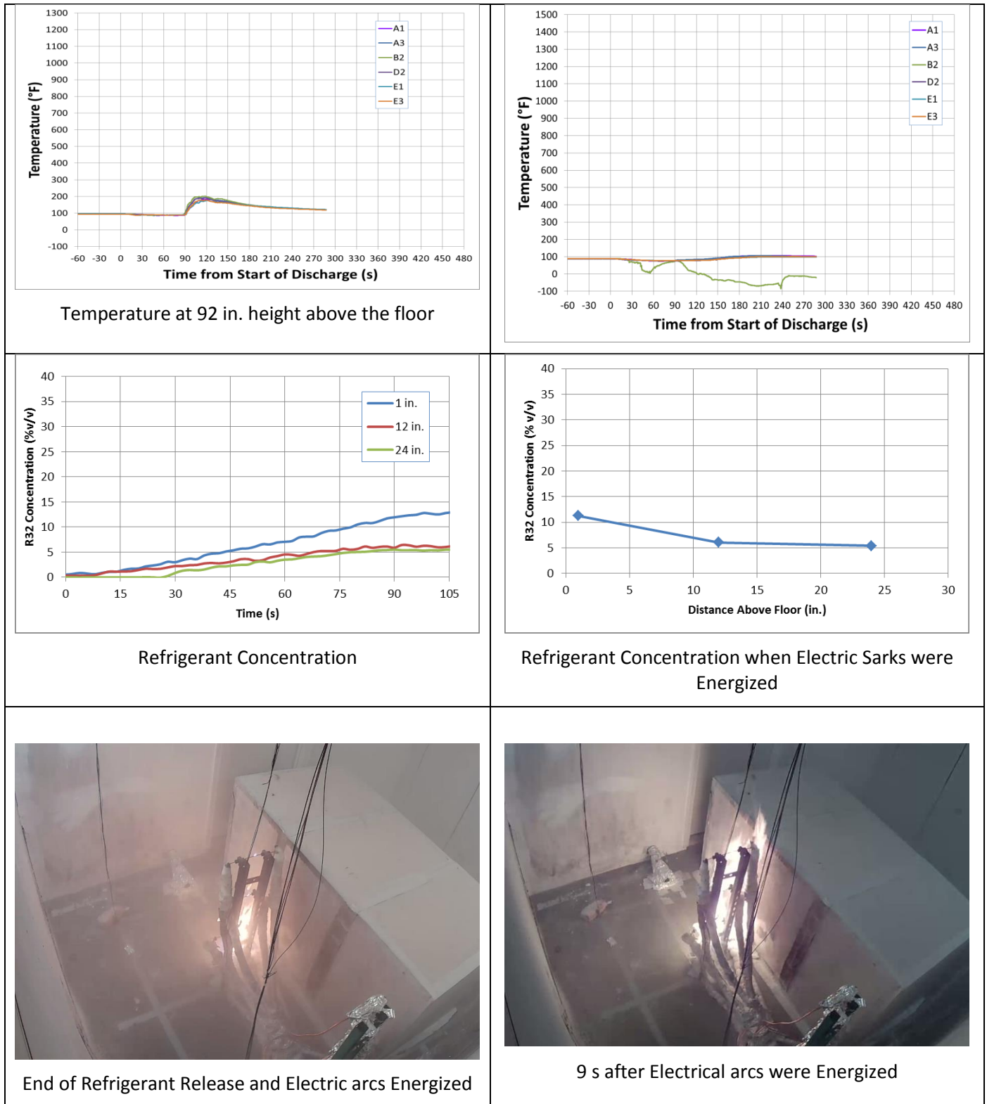
Figure 50 – Data from Cal16
