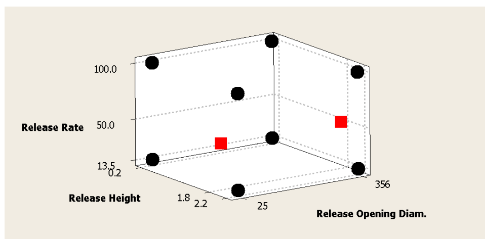
Figure 33 – Test Matrix. The red squares are on the 25 and 356 mm Release Opening Diameter face of the cube.
