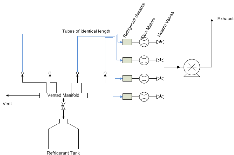
Figure 25 – Setup for calibration of refrigerant sensors
