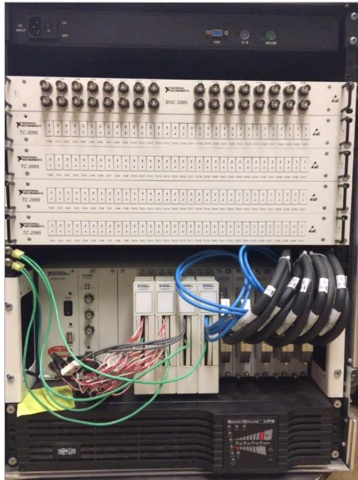
Figure 160 - DAS\NI Data Acquisition System
