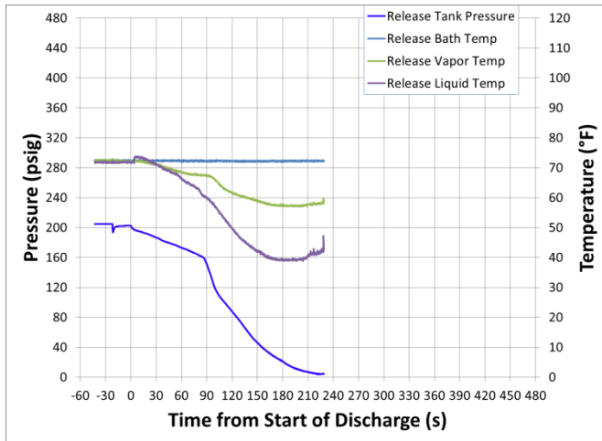
Pressure and Temperature in Release Tank
