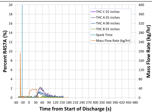
Refrigerant Concentration (see notes)
