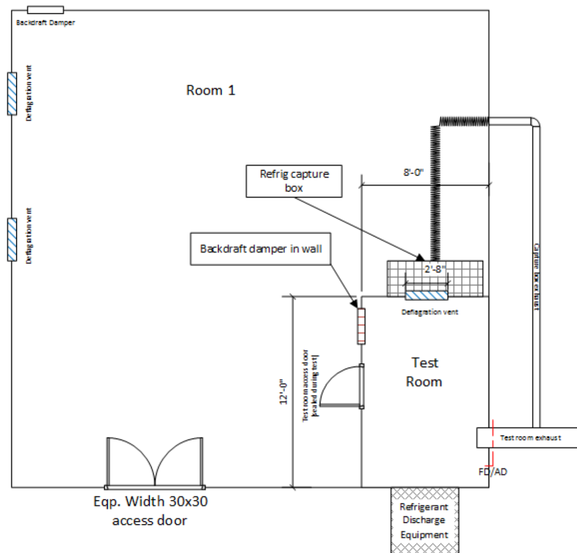
Figure 12 – Task 1 room design
