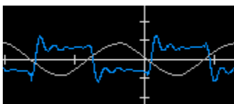
Figure 15 – Trace of current (smooth sine wave) and voltage in an electric arc
