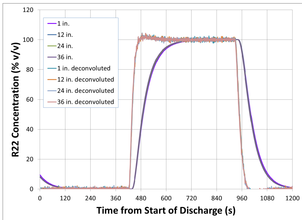
Figure 26 – Accounting for Refrigerant Sensor Response Time and Transport Delay
