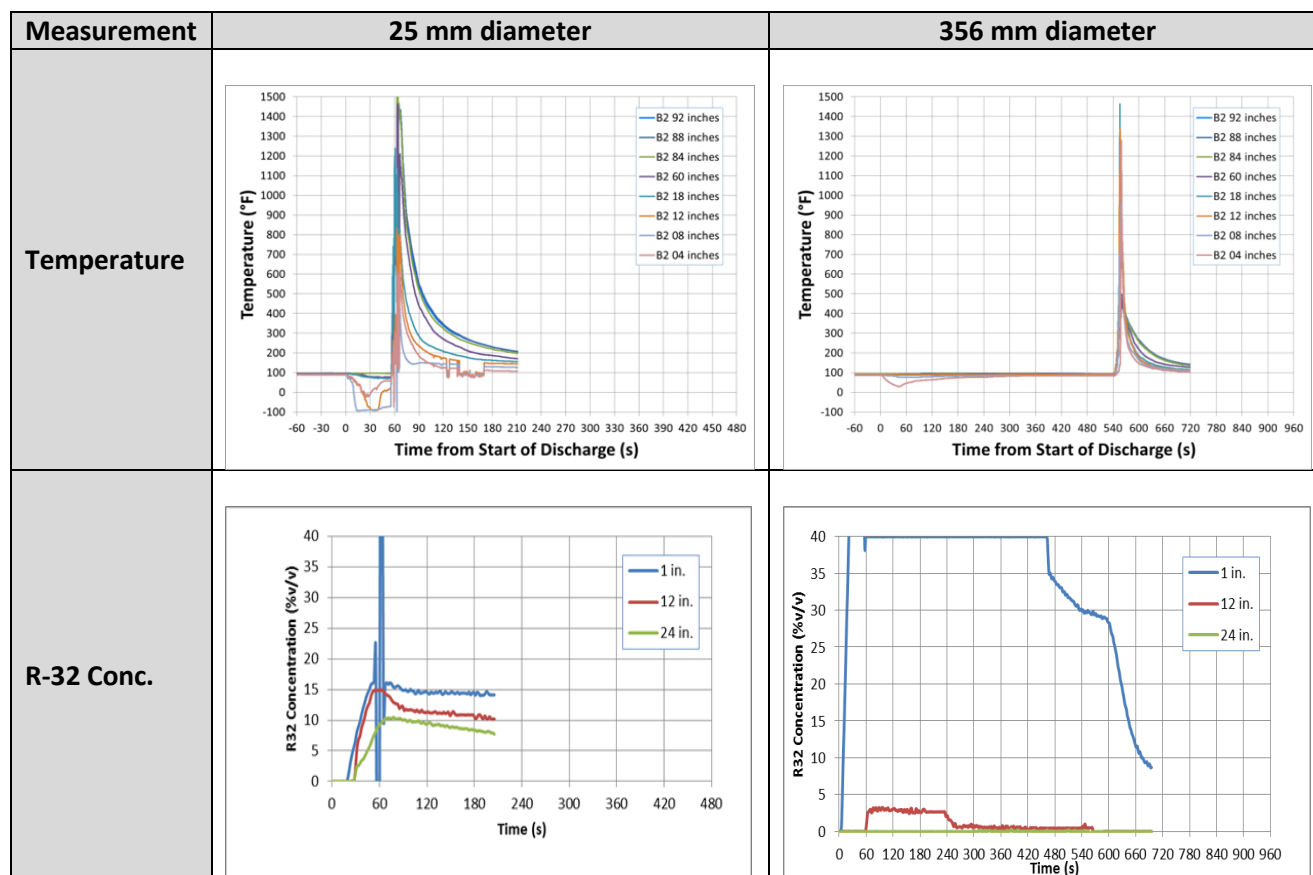
Figure 40 – Influence of Refrigerant Release Opening Diameter (Release rate: 100 g/s; 0.2m height)
