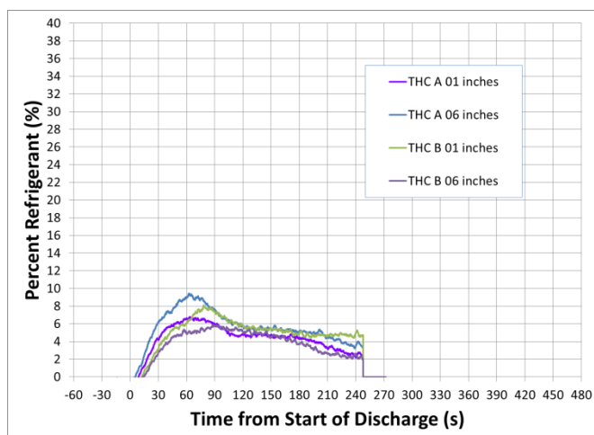
Refrigerant Concentration PTAC06
