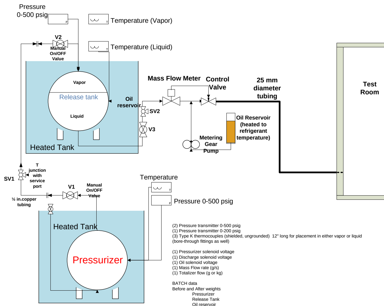
Figure 17 - Refrigerant release methodology with lubricating oil
