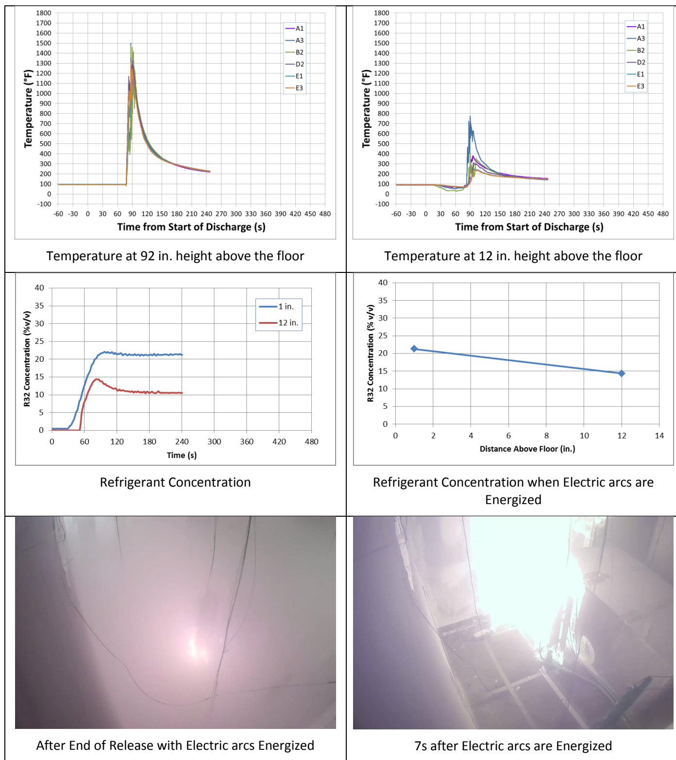
Figure 66 – Data for PB01
