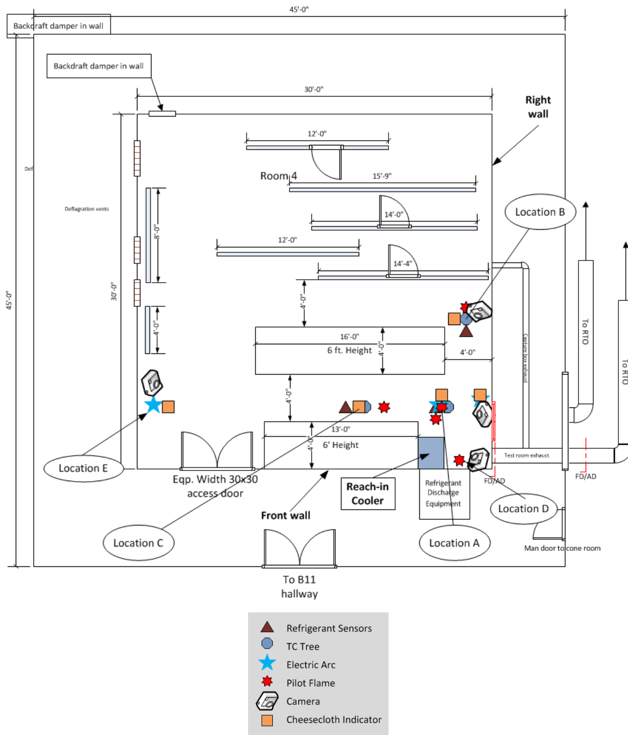
Figure 106 – Reach-in Cooler Test Setup
