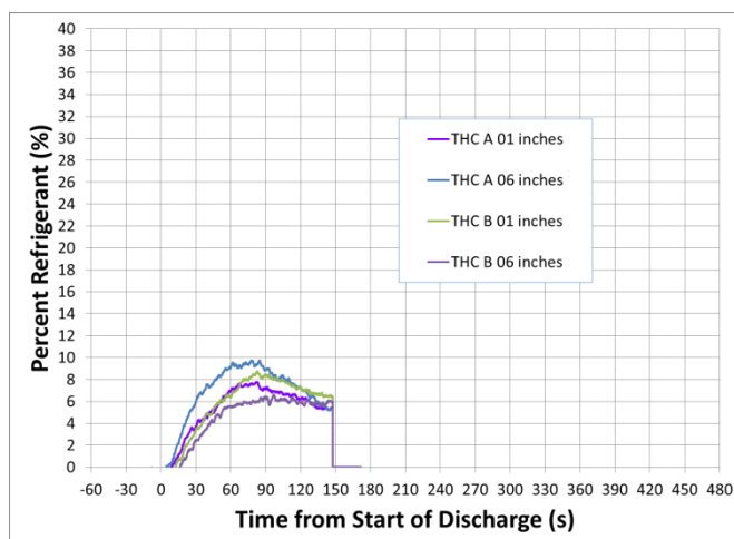
Refrigerant Concentration PTAC08
