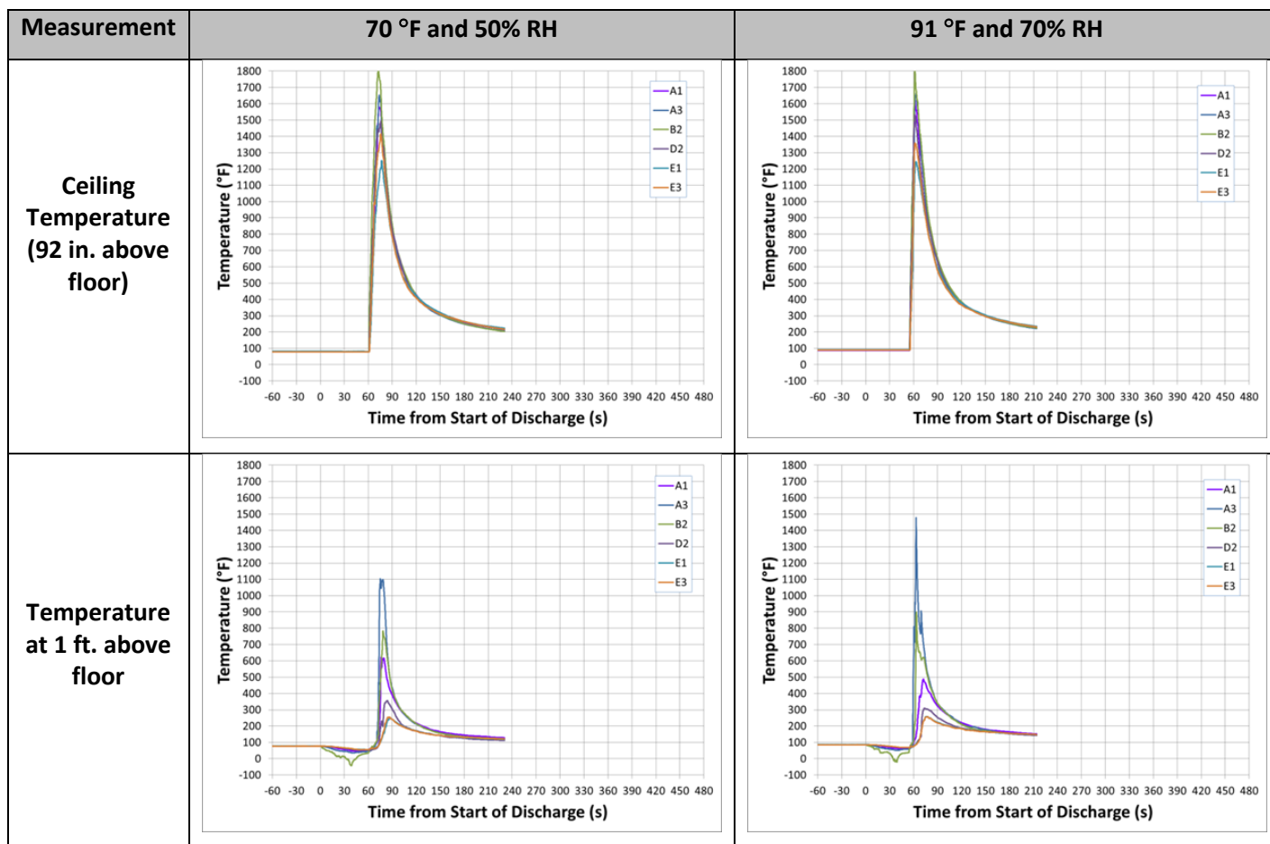
Figure 53 – Influence of Temperature and Humidity for R-452B Refrigerant
