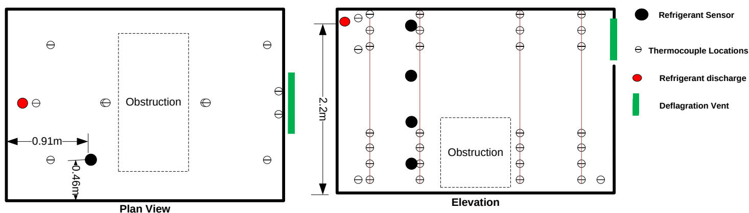
Figure 28 – Test Room Leakage Characterization
