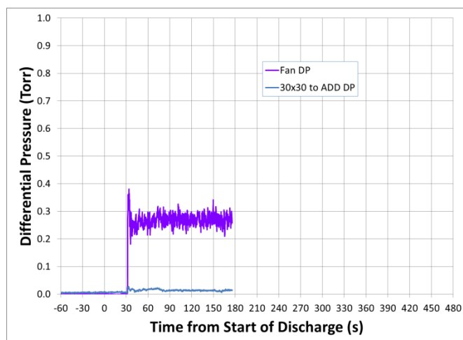
Room and Blower Differential Pressure
