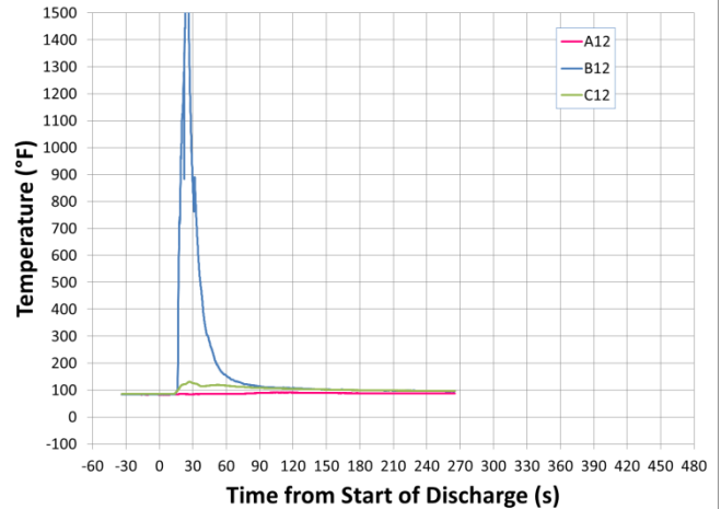
Highest temperature: Temperature 12 in. height above the floor at Location B
