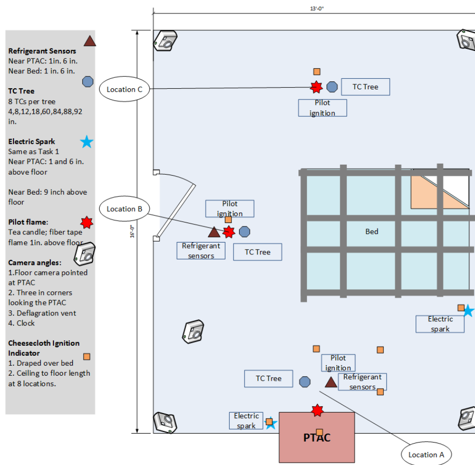
Figure 87 – Larger view of motel room detail
