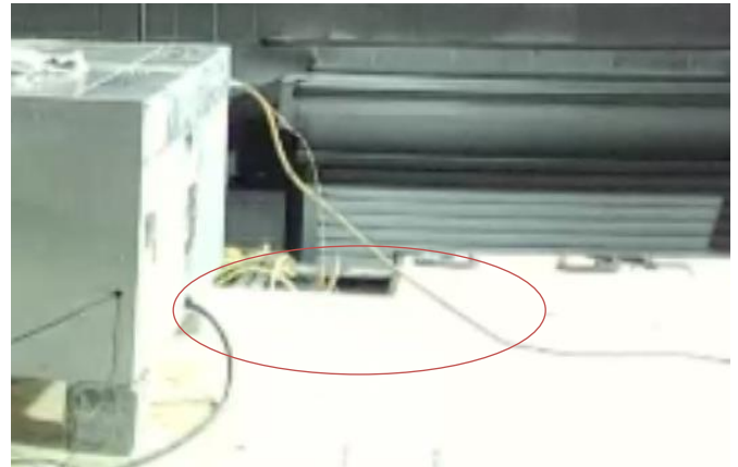
Condensate Drain on RTU showing a barely visible mist escaping through this route. The power cable for the fan motor was routed through the condensate drain. The mist is more visible on the video of this test.
