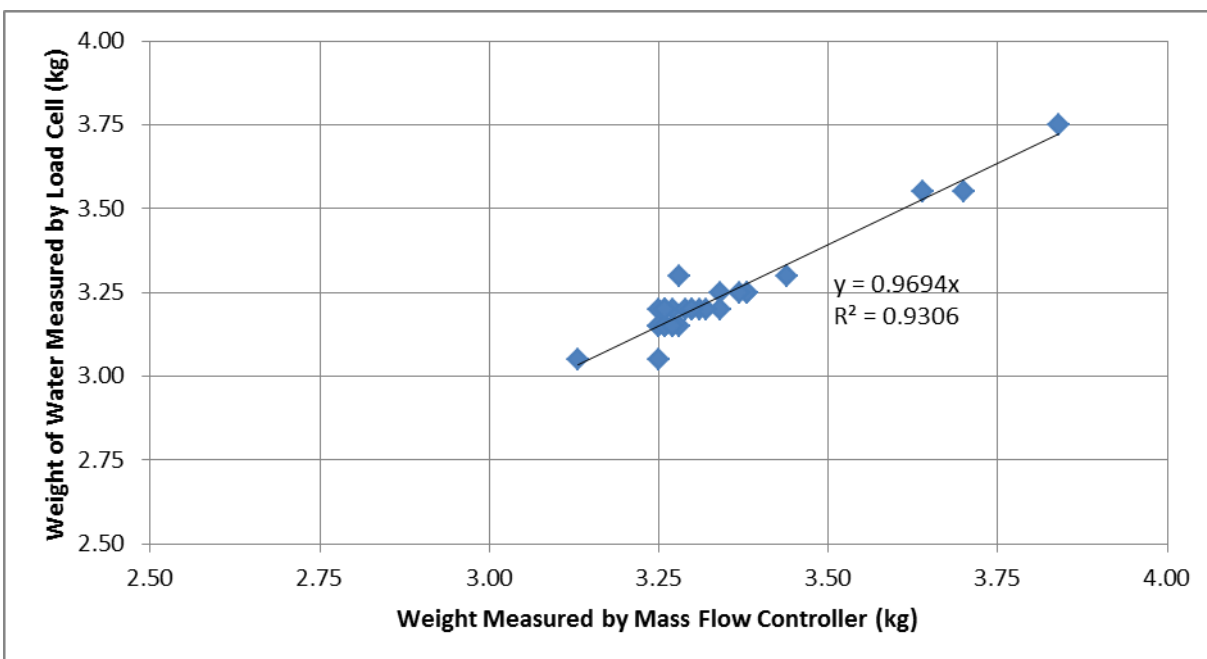
Figure 21 - Mass flow Controller Versus Load Cell
