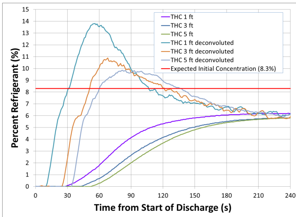
Figure 30 – Deconvoluted concentrations for the room leakage test
