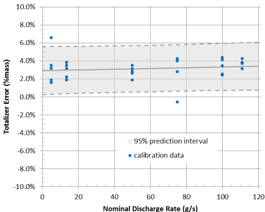
Figure 23 –Totalizer Error versus Nominal Discharge Rate
