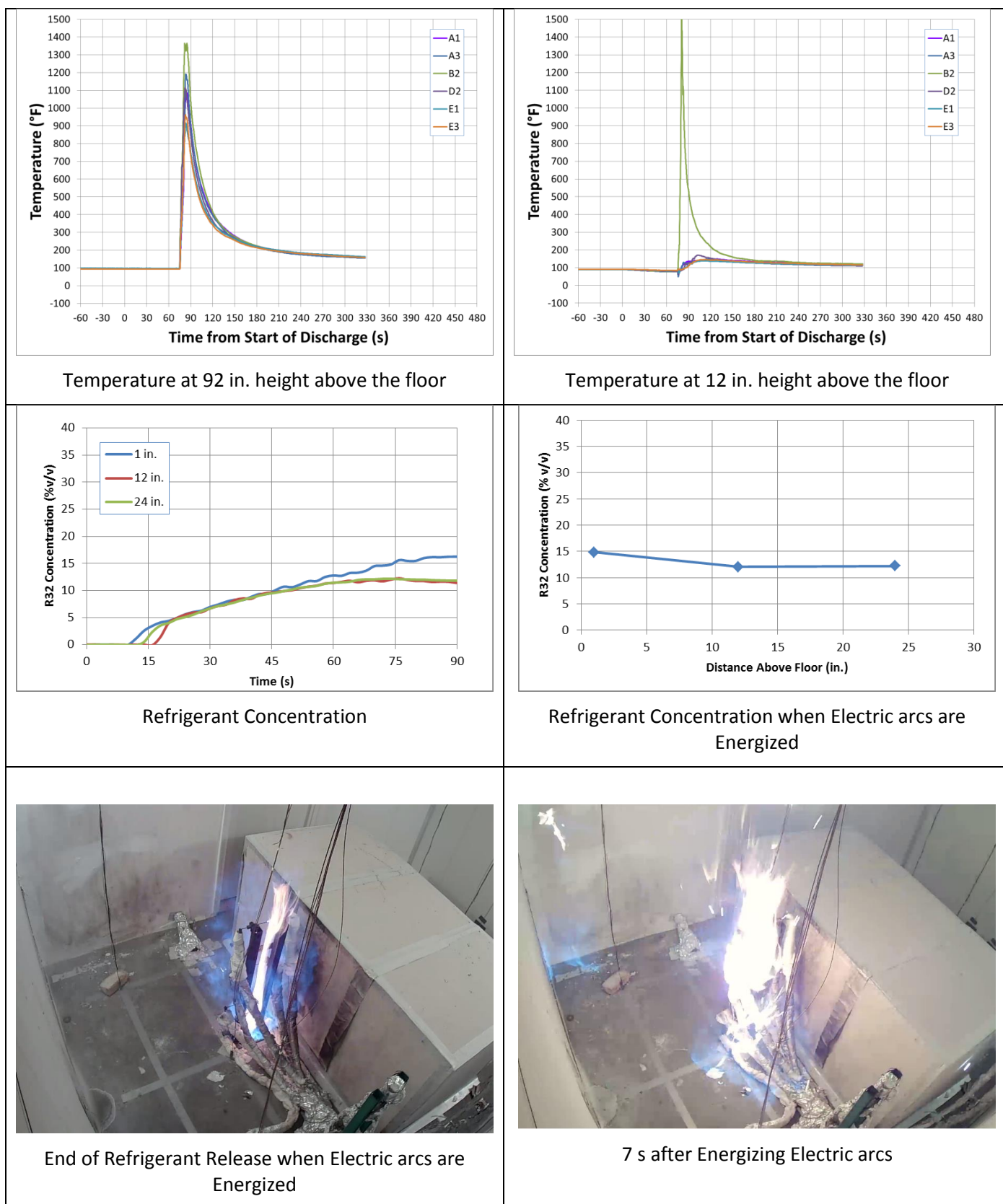
Figure 49 – Data from Cal13
