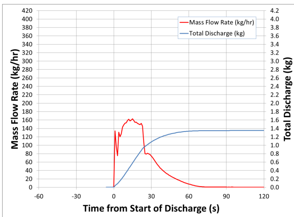
Figure 145 - Refrigerant Release Rate (RES08 test)
