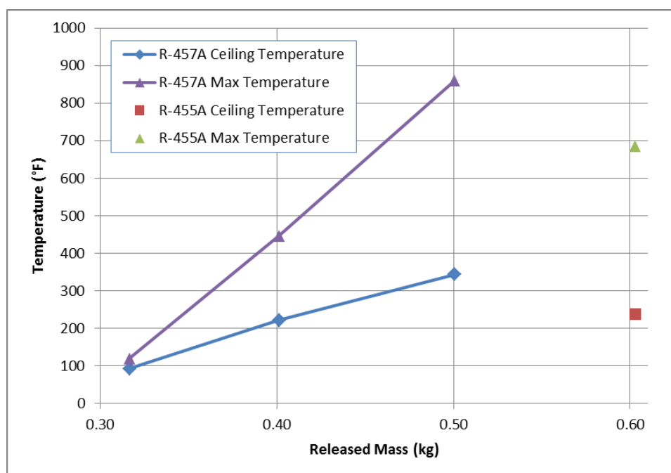
Figure 107 – Maximum Temperatures and Ceiling Temperatures
