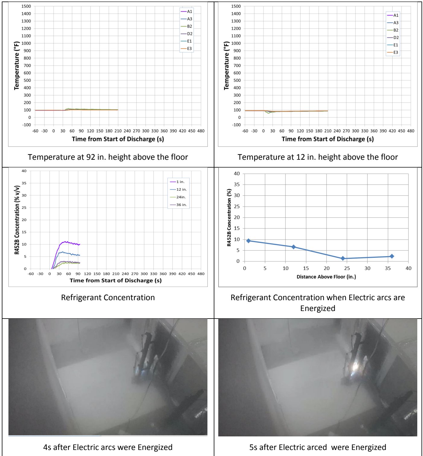
Figure 74 – Data for PB11
