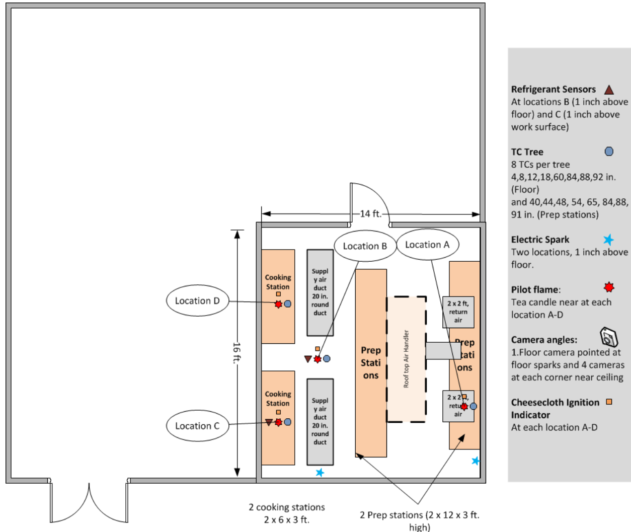
Figure 112 – Commercial Kitchen Layout within the 30'x30' test room
