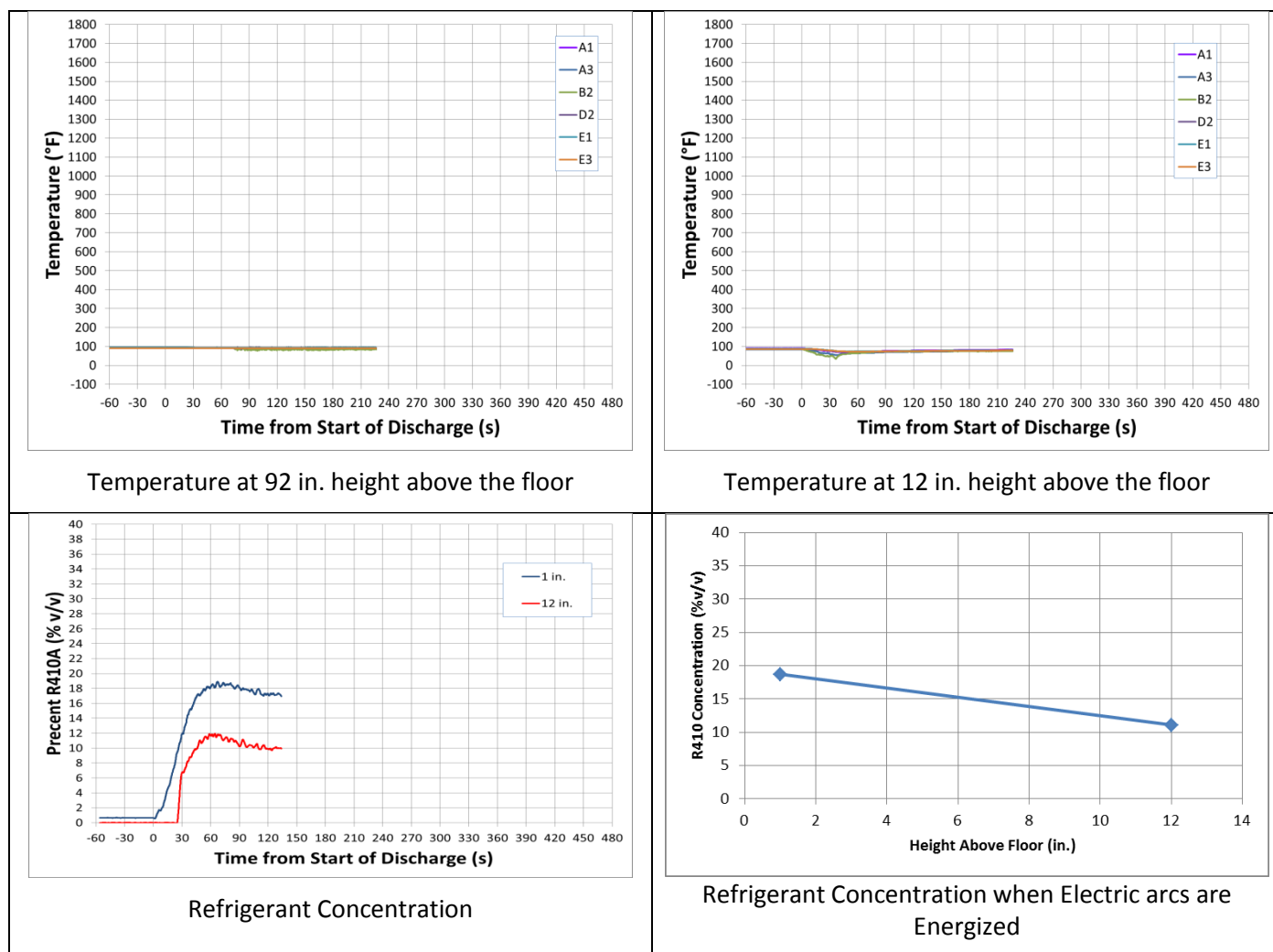
Figure 65 – Data for PA04
