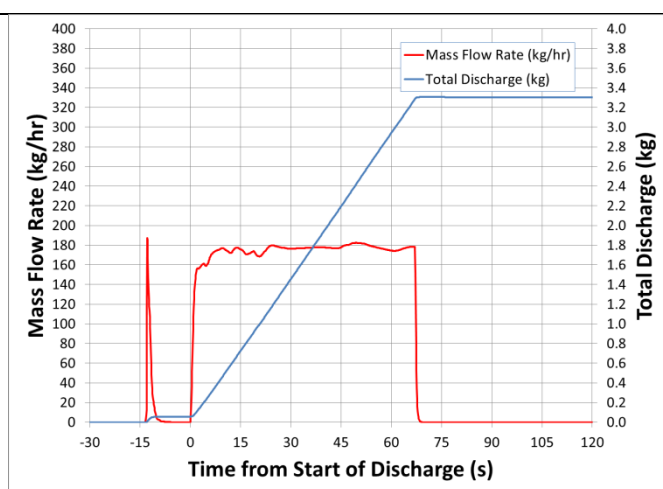
Refrigerant Release Rate
