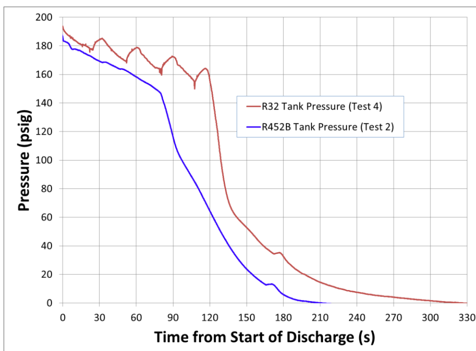
Figure 151 – Comparison of Release Tank Pressures during Hermetic Electrical Pass-Through Terminal Failure Tests
