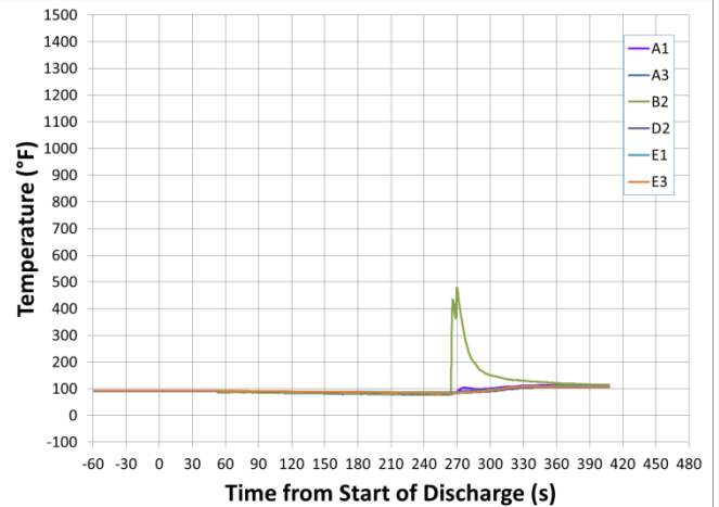
Temperatures at 12 in. height above the floor
