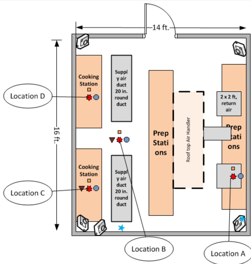
Figure 113 – Larger view of commercial kitchen detail
