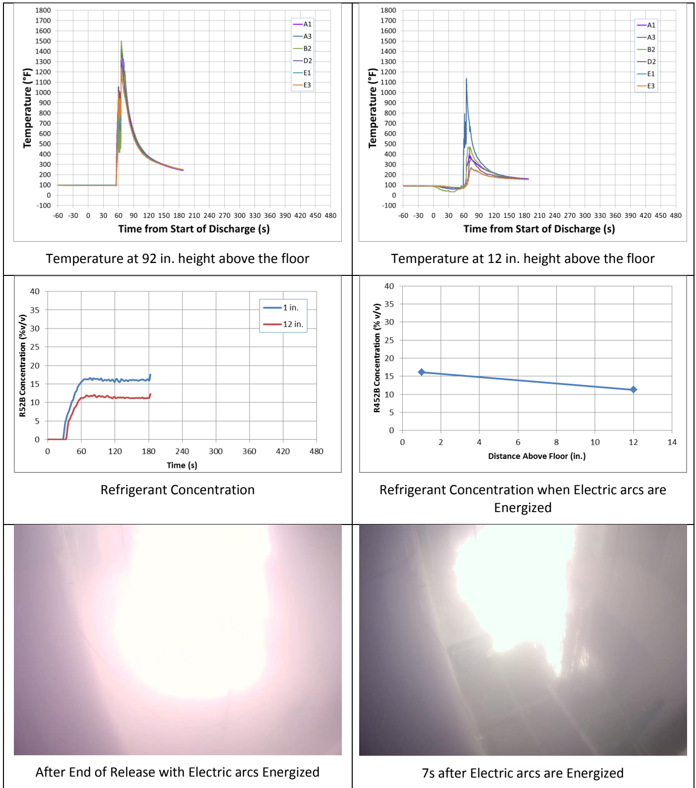
Figure 67 – Data for PB02
