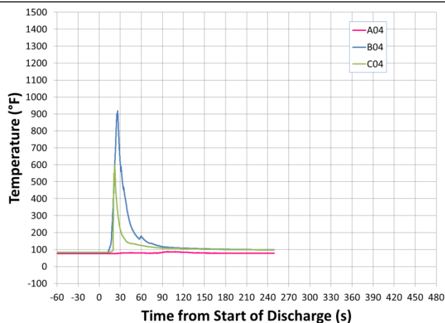
Highest temperature: Temperature 4 in. height above the floor
