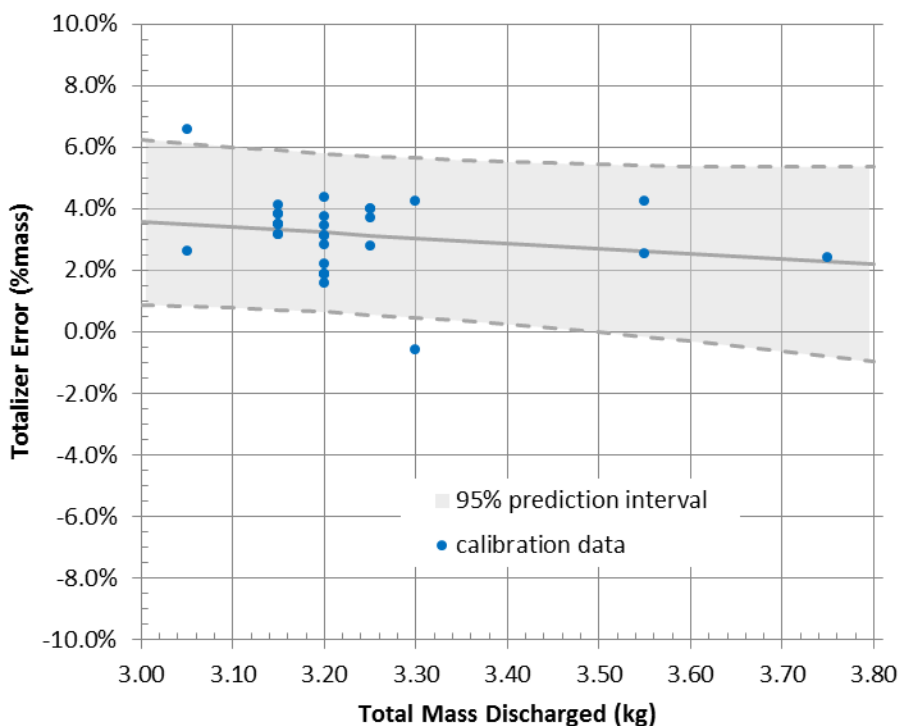
Figure 22 – Totalizer Error versus Total Mass Discharged
