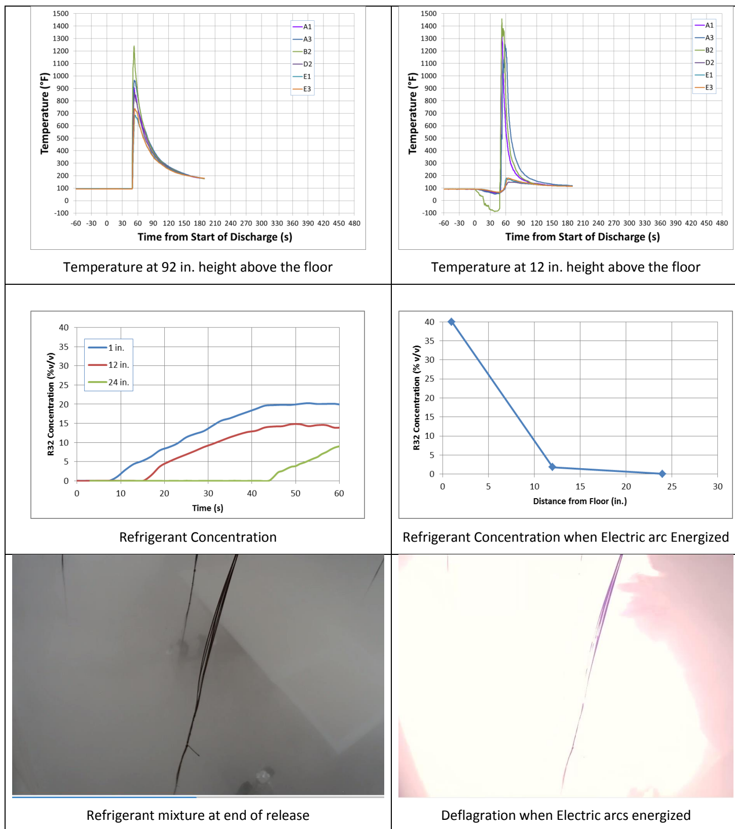
Figure 45 – Data from Cal09
