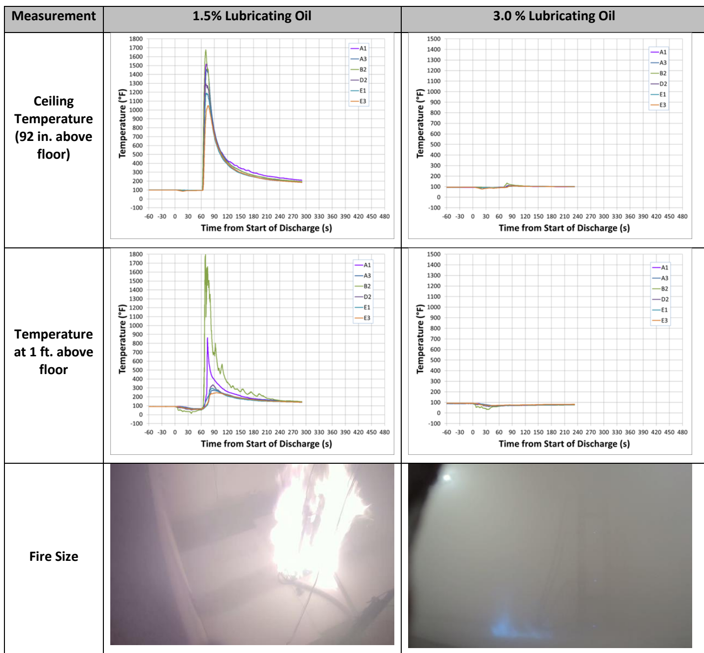
Figure 60 – Comparison of Results for R-32 Refrigerant with Lubricating Oil
