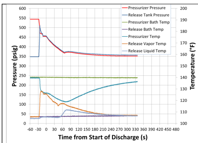
Pressure and Temperature of Release and Pressurizer Tanks
