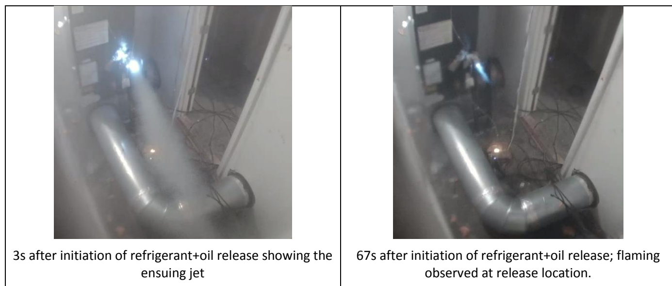
Figure 146 - Test Results for Residential A/C Res08
