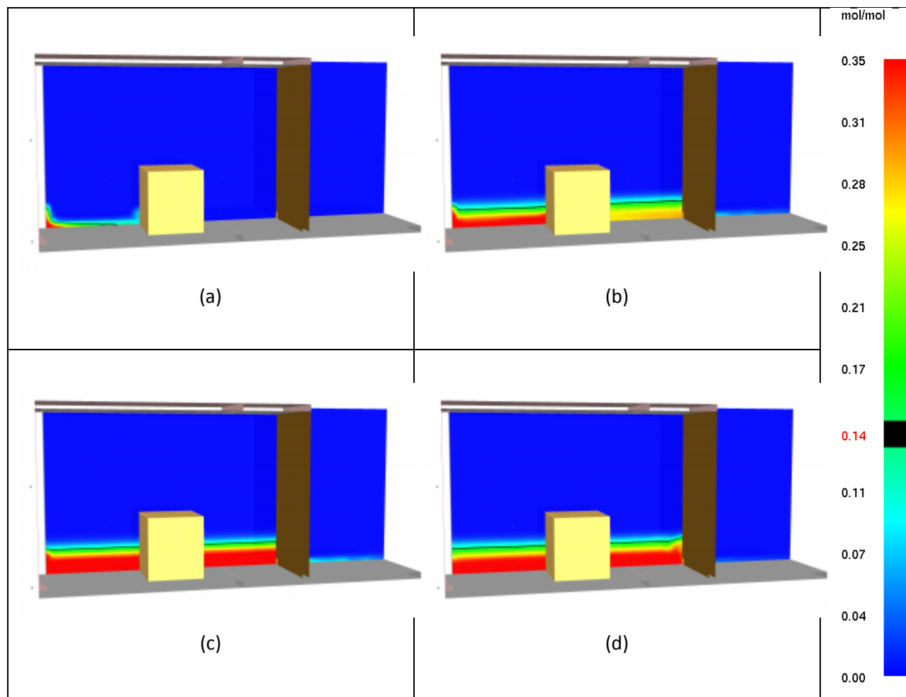
Figure 9 – Still images from FDS simulation 8 at times: (a) 5 s (b) 120 s (c) 240 s (d) 300 s
