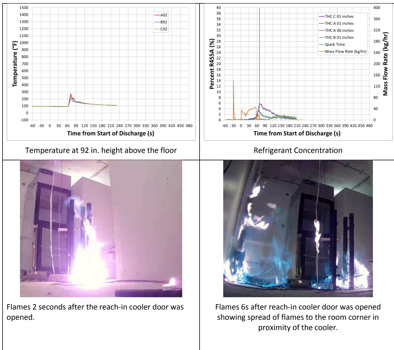
Figure 108 – Test Results for Reach-in Cooler - Cooler01
