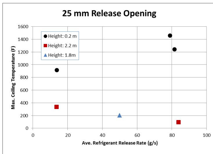
Figure 35 – Maximum Temperature Refrigerant Released from 25 mm diameter opening
