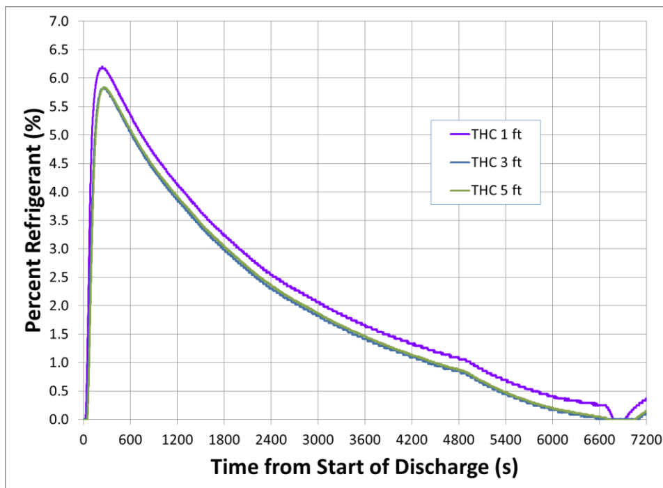
Figure 29 – Refrigerant Concentration: Leakage Test
