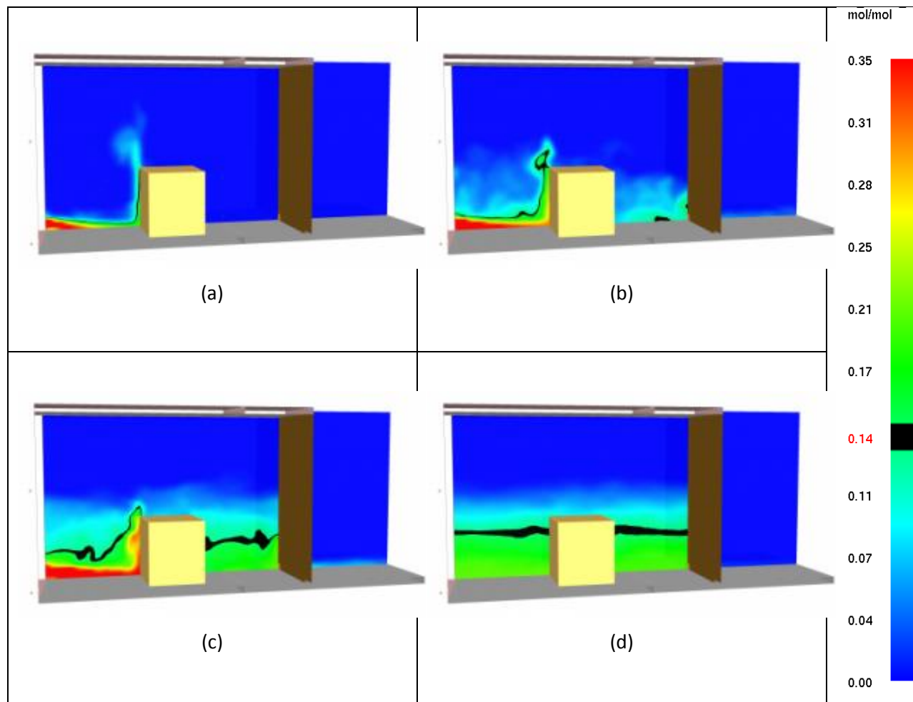
Figure 6 – Still images from FDS simulation 5 at times: (a) 5 s (b) 15 s (c) 30 s (d) 90 s
