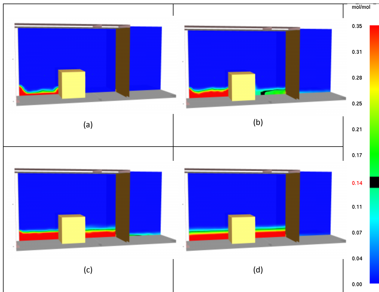
Figure 7 – Still images from FDS simulation 7 at times: (a) 5 s (b) 15 s (c) 30 s (d) 90 s
