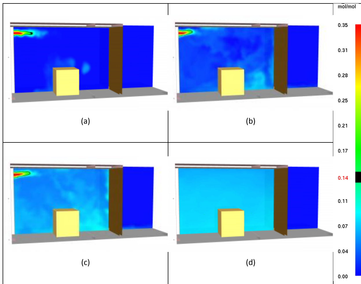
Figure 2 – Still images from FDS simulation 1 at times: (a) 5 s (b) 15 s (c) 30 s (d) 90 s
