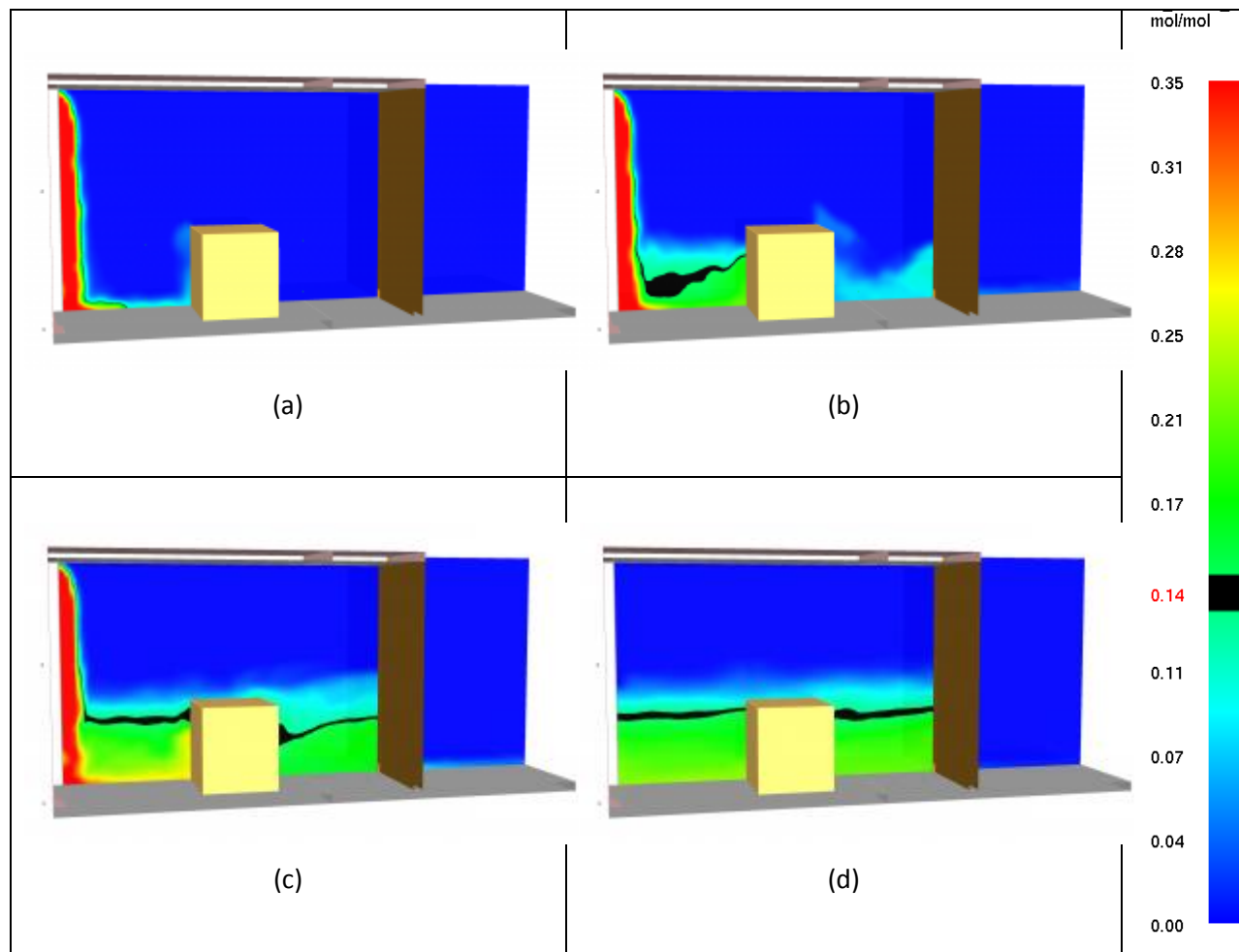
Figure 3 – Still images from FDS simulation 3 at times: (a) 5 s (b) 15 s (c) 30 s (d) 90 s
