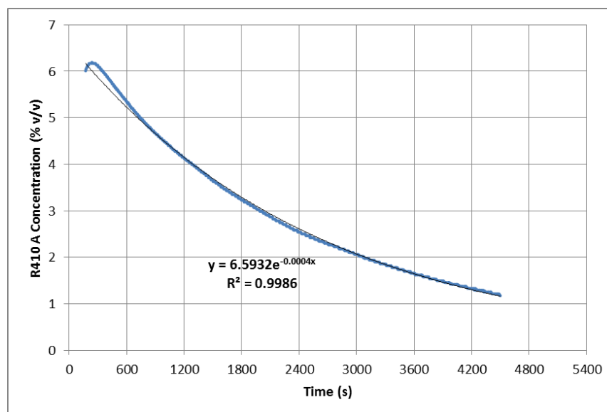
Figure 31 – Refrigerant Concentration Decay with Deflagration Vent Closed
