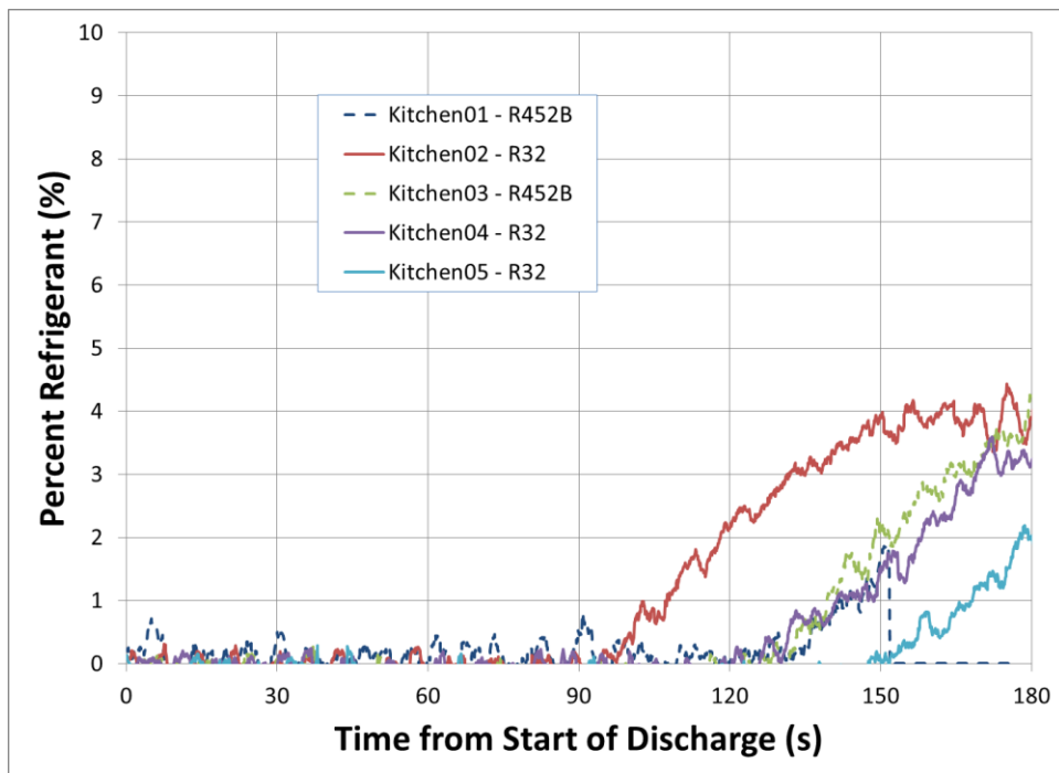
Figure 118 - Refrigerant Concentration Location C (1 inch above the work surface)
