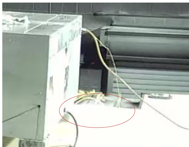
Condensate Drain on RTU showing a mist escaping through this route. The power cable for the fan motor was routed through the condensate drain.
