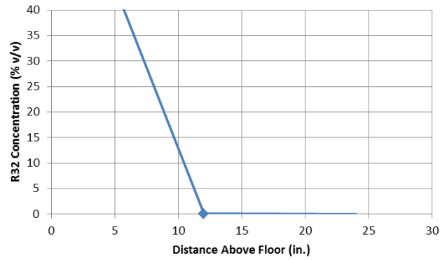
Refrigerant Concentration When Electric arcs are Energized at 60s (first attempt)
