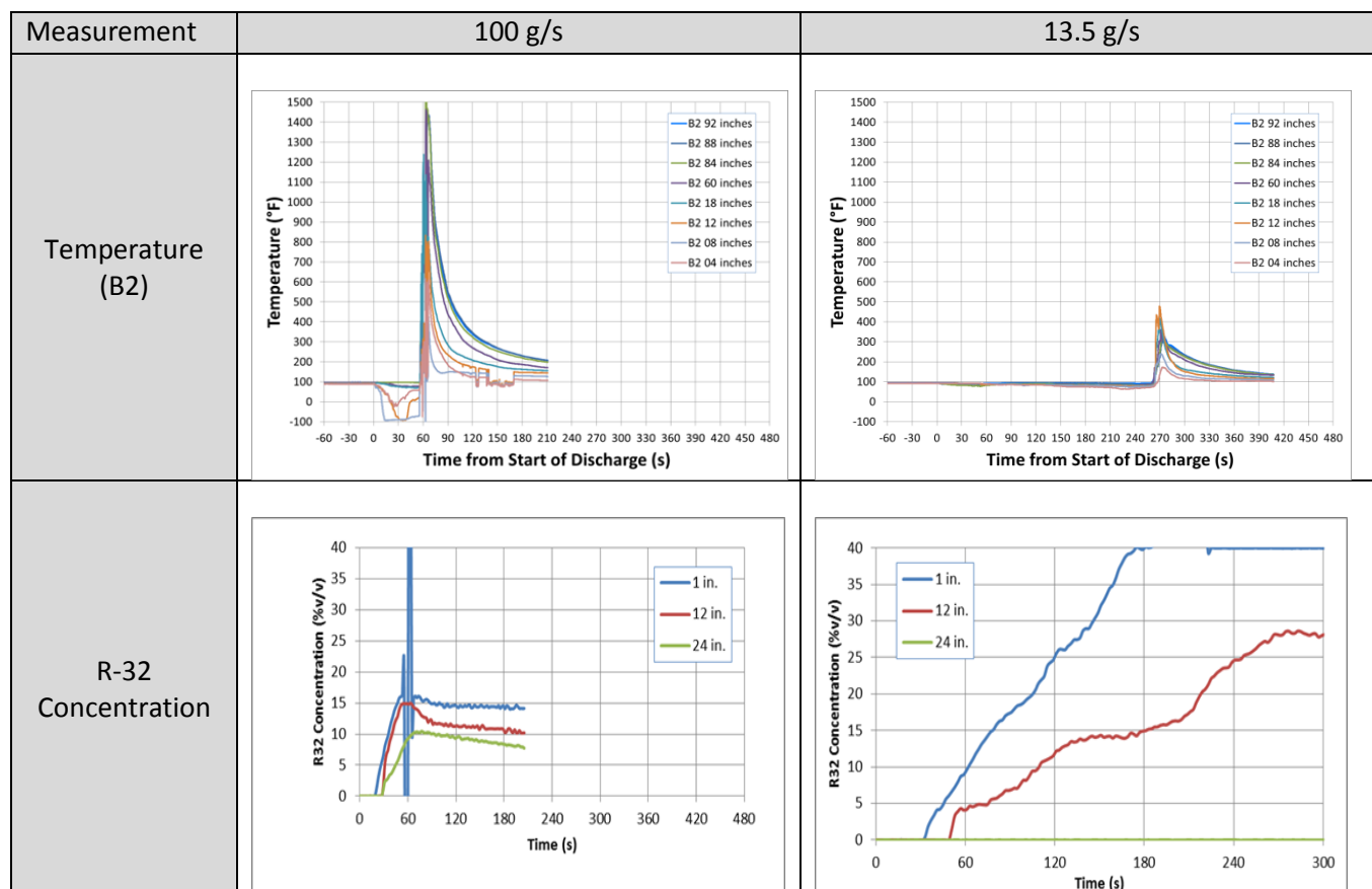
Figure 36 – Influence of Refrigerant Release Rate (100 g/s from 0.2m height through a 25 mm diameter opening)
