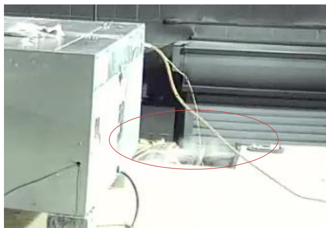
Condensate Drain on RTU showing a mist escaping through this route. The power cable for the fan motor was routed through the condensate drain.
