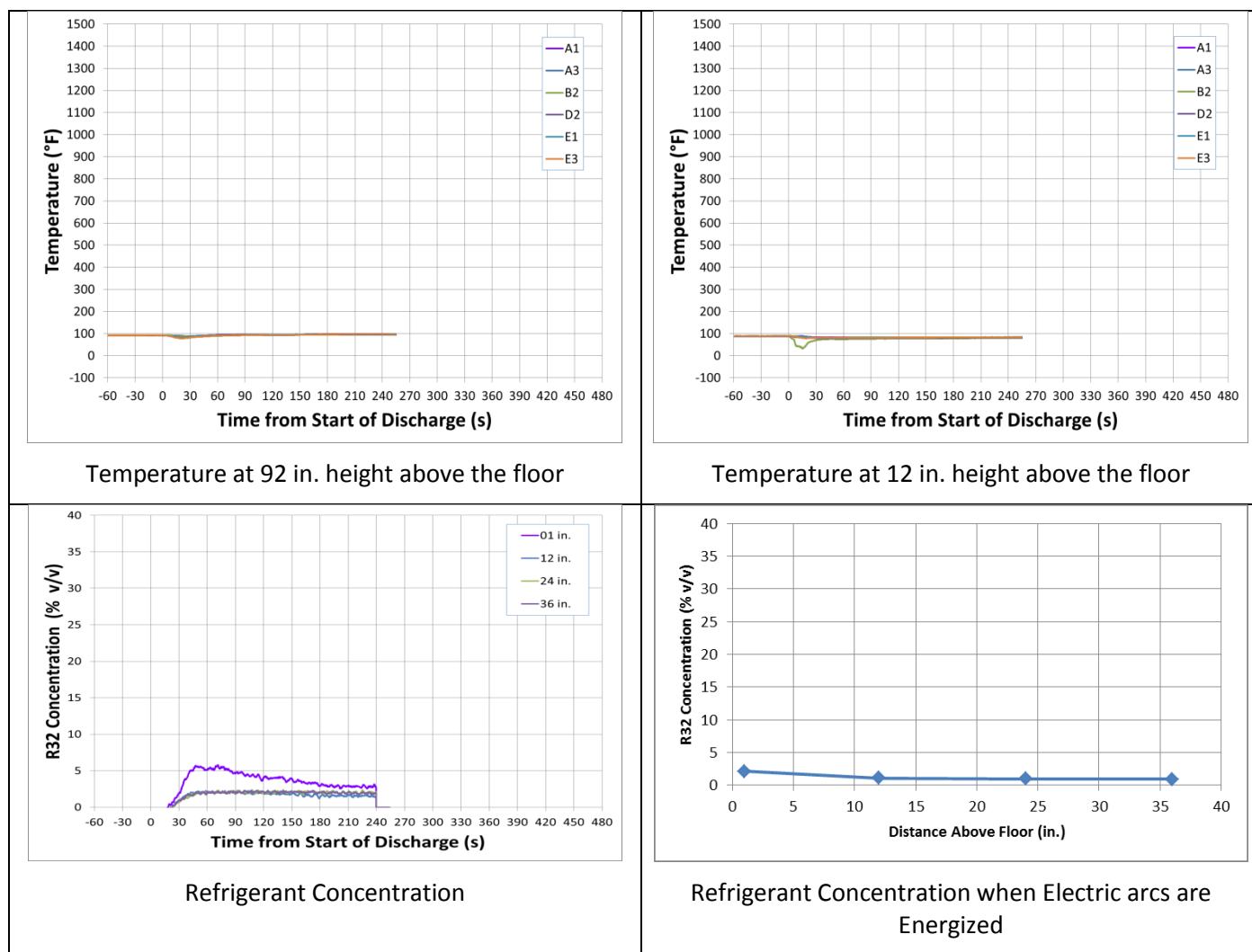
Figure 71 – Data for PB08
