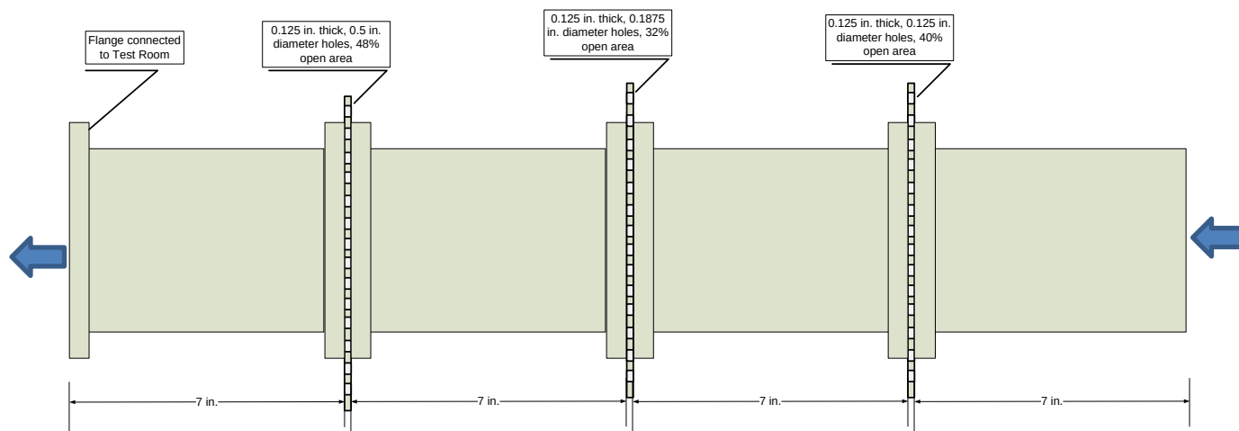
Figure 18 – 14 in. Release Duct Assembly
