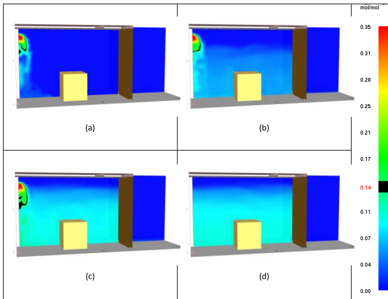
Figure 4 – Still images from FDS simulation 2 at times: (a) 5 s (b) 120 s (c) 240 s (d) 300 s
