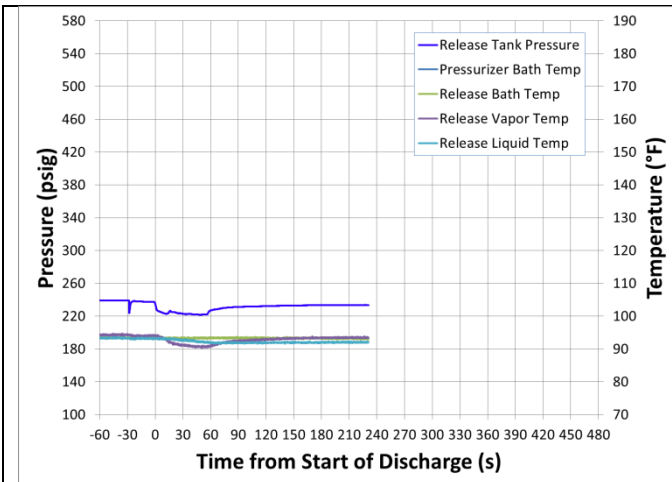
Pressure and Temperature in Pressurizer and Release Tanks
