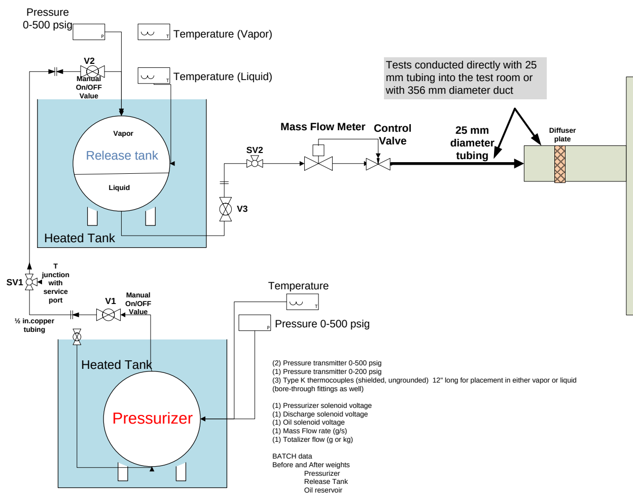
Figure 16 – Refrigerant release methodology without lubricating oil
