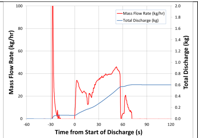
Refrigerant Release Rate
