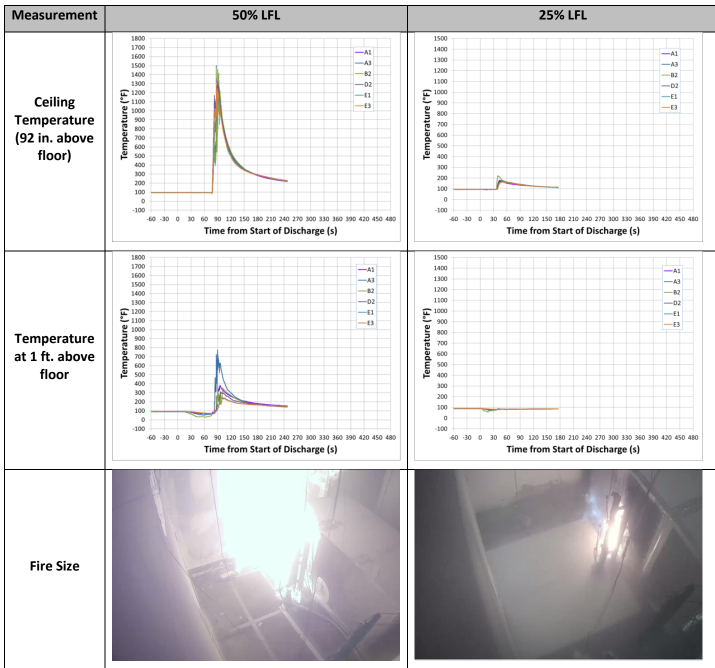
Figure 59 - Comparison of Released Refrigerant Quantity for R-32 Refrigerant
