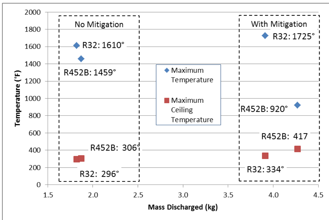
Figure 138 - Peak temperatures near floor and at ceiling
