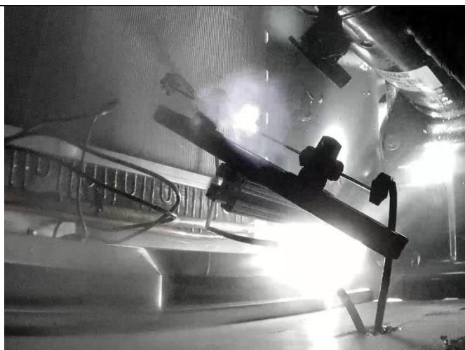
Displacement of Molded Plug and Refrigerant Release (19s after release start)
