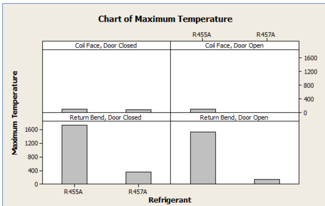
Figure 127 – Chart of Maximum Temperature versus Discharge Location and Door Position
