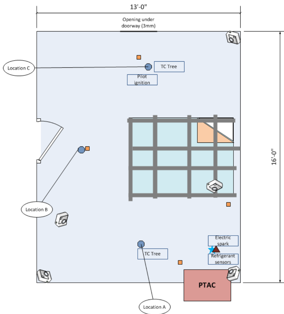
Figure 104 – Instrumentation for MPTAC01
