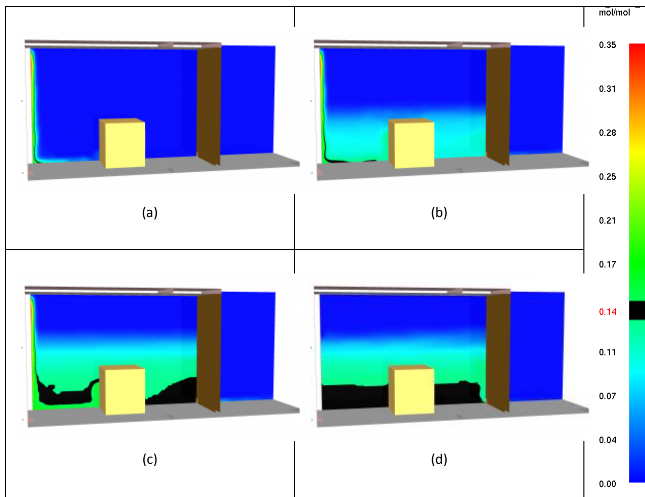
Figure 5 – Still images from FDS simulation 4 at times: (a) 5 s (b) 120 s (c) 240 s (d) 300 s
