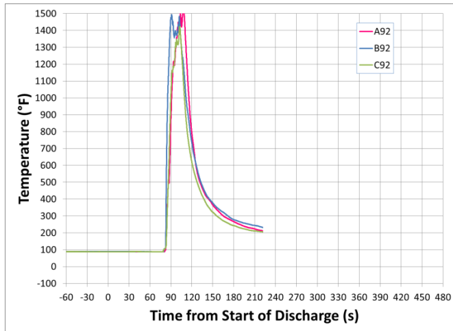
Temperature at 92 in. height above the floor
