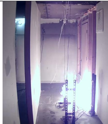
Flames 20s after refrigerant release; flames moves toward the return air grill.
