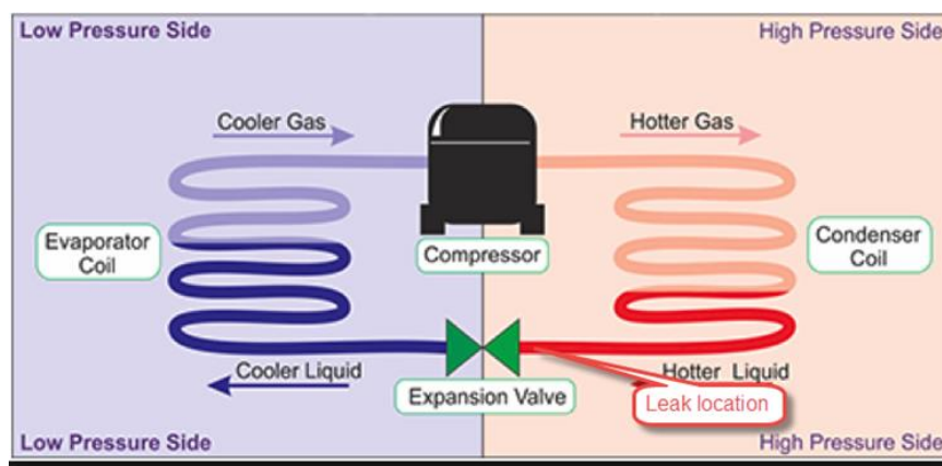
Figure 10 – Refrigeration Leak Scenario
