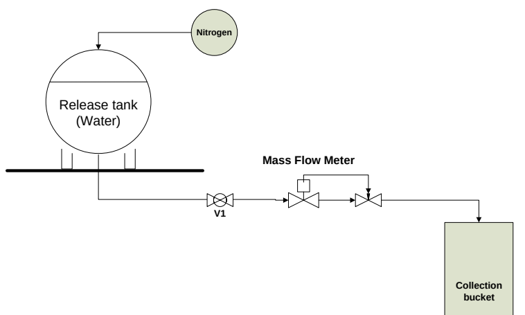
Figure 20 – Test Set up for Response Time and Validation of Mass Flow Meter and Controller
