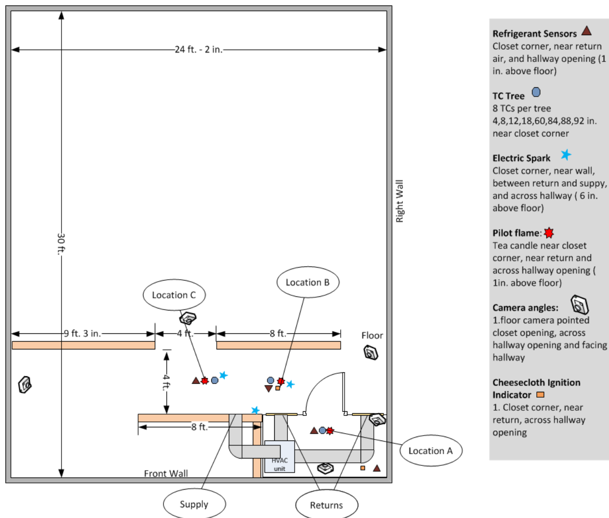
Figure 135 – Residential Scenario Test Setup
