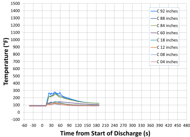
Temperature at Location C
