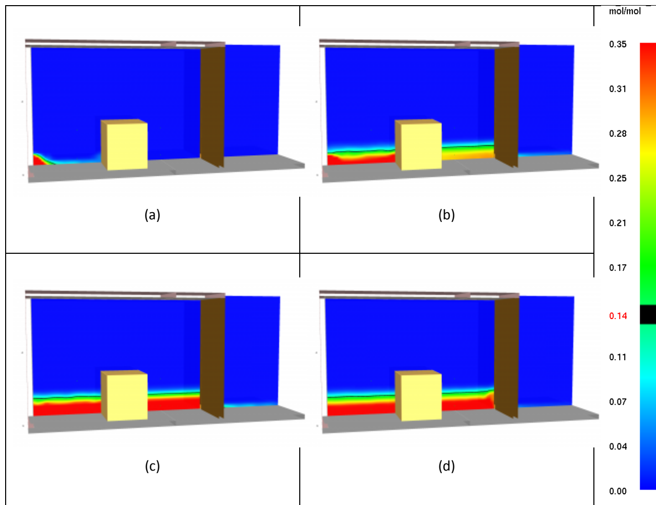
Figure 8 – Still images from FDS simulation 6 at times: (a) 5 s (b) 120 s (c) 240 s (d) 300 s
