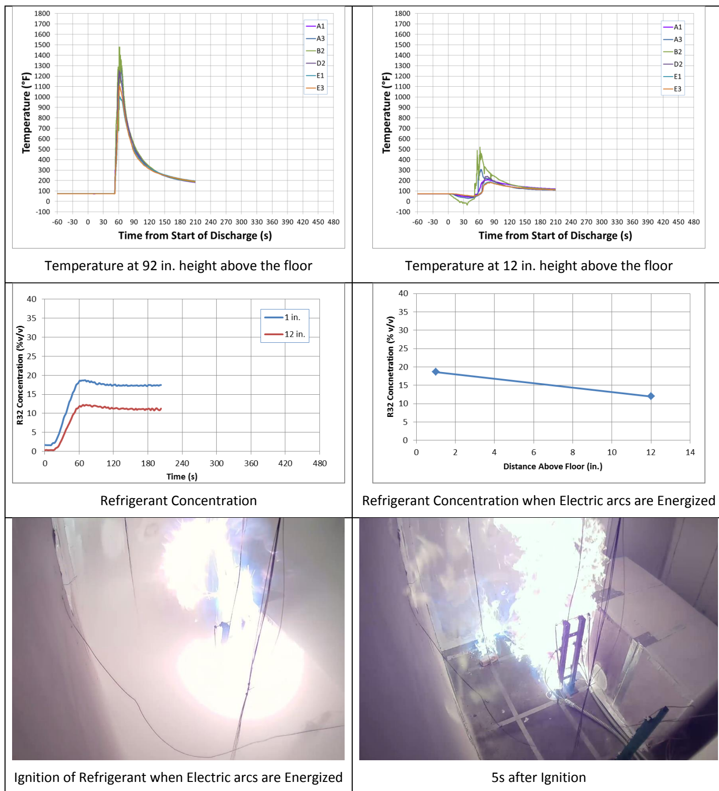
Figure 63 – Data for PA03
