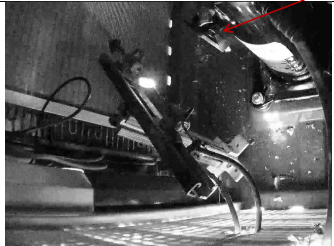
Displacement of Molded Plug approximately 14s after release
