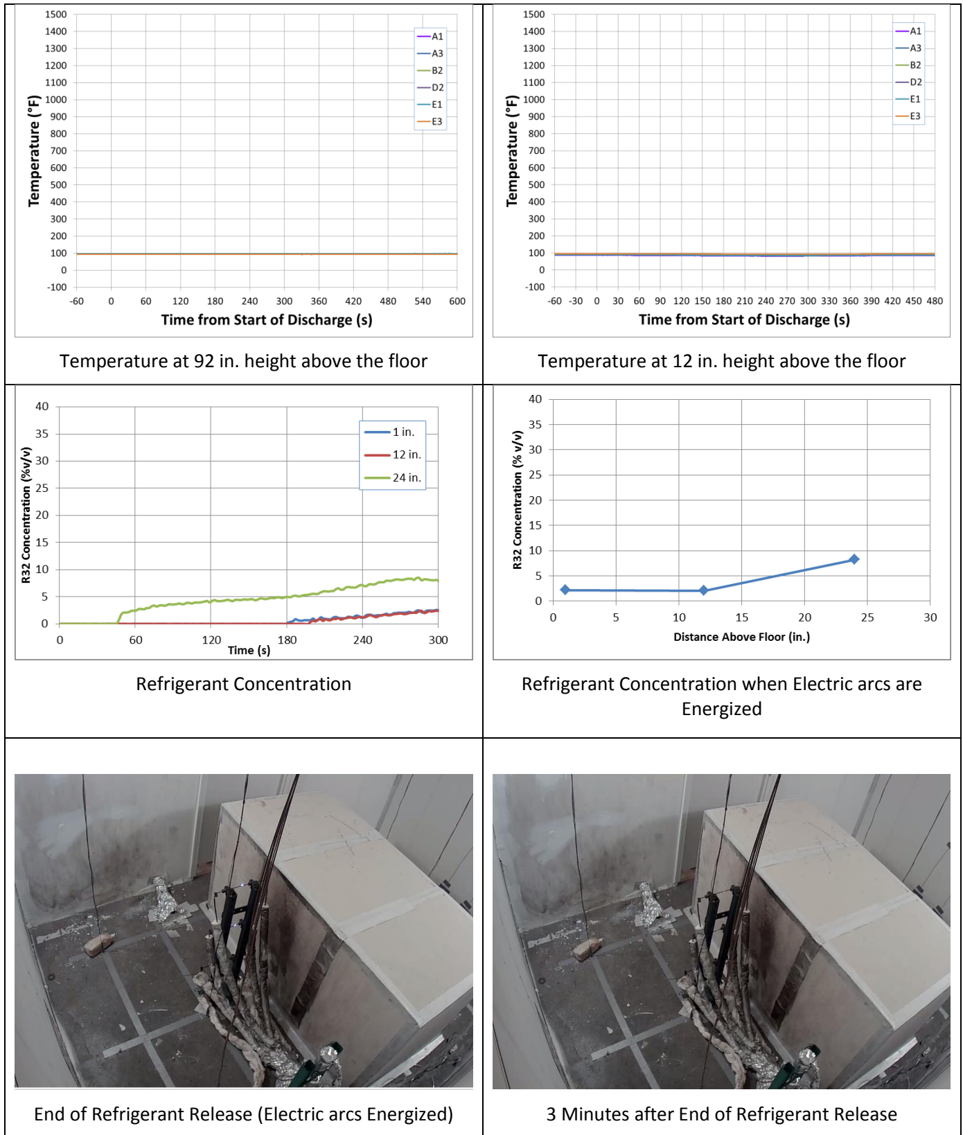
Figure 48 – Data from Cal012
