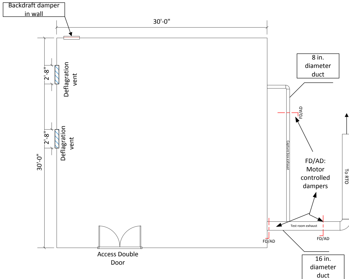
Figure 11 Conditioned Test facility
