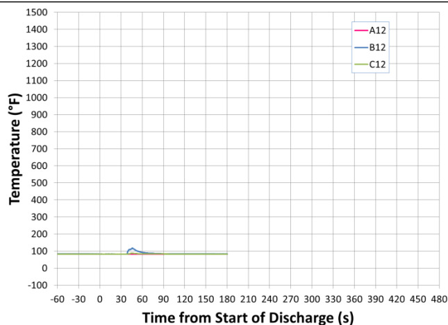
Highest temperature: Temperature 12 in. height above the floor
