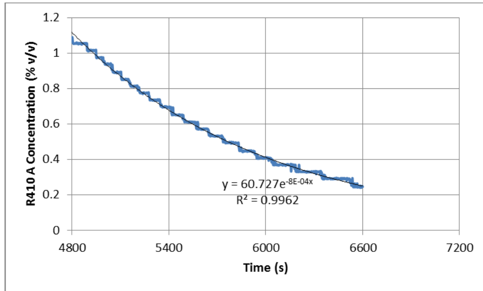
Figure 32 - Refrigerant Concentration Decay with Deflagration Vent Open
