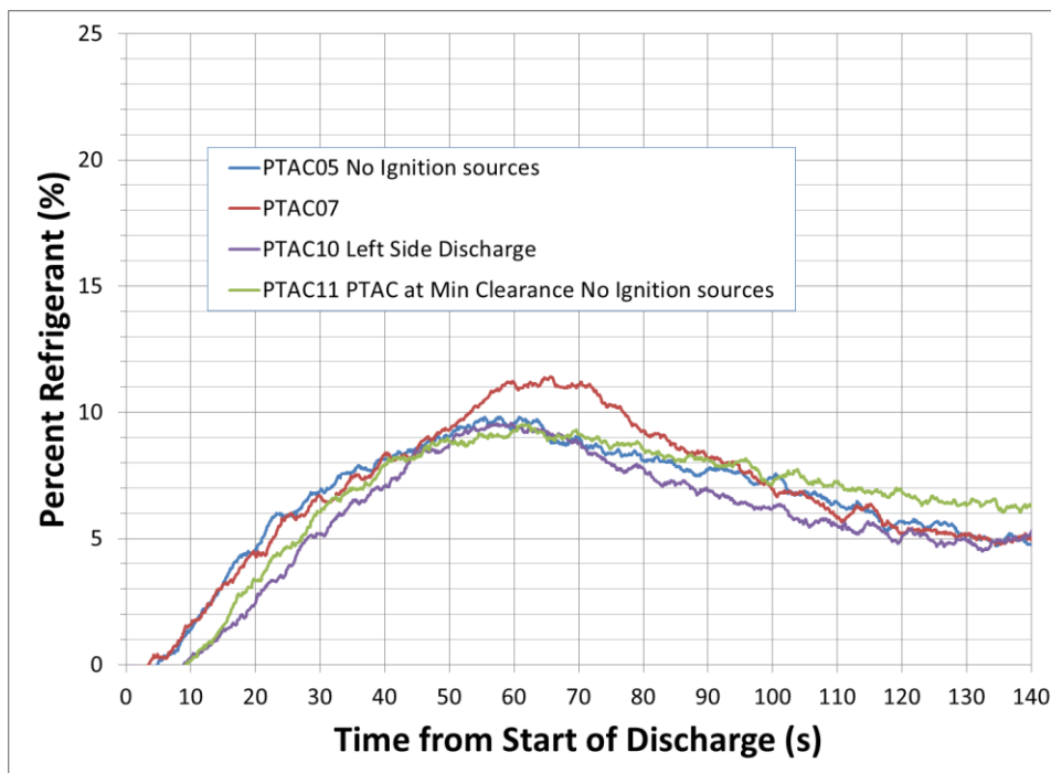
Figure 92 – Comparison of R-452B concentrations
