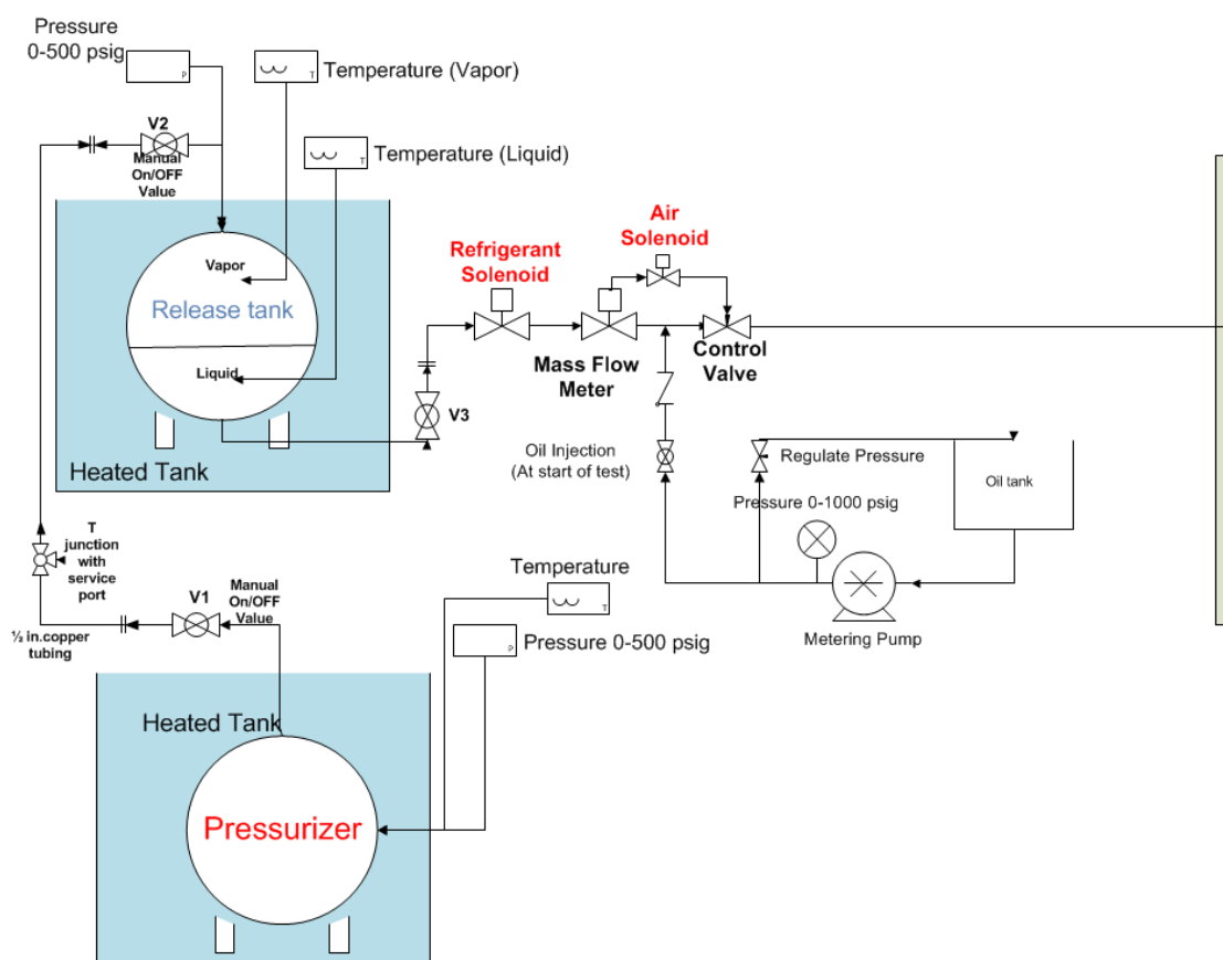
Figure 84 –Refrigerant Release and Oil Injection system with remotely operated solenoid valves
