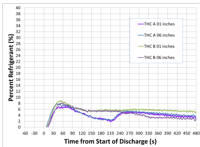
Refrigerant Concentration PTAC11
