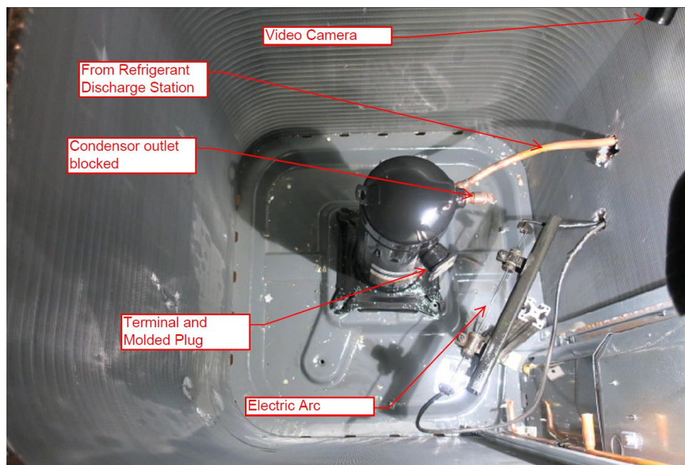
Figure 150 – Interior Arrangement of Condensing Unit Components
