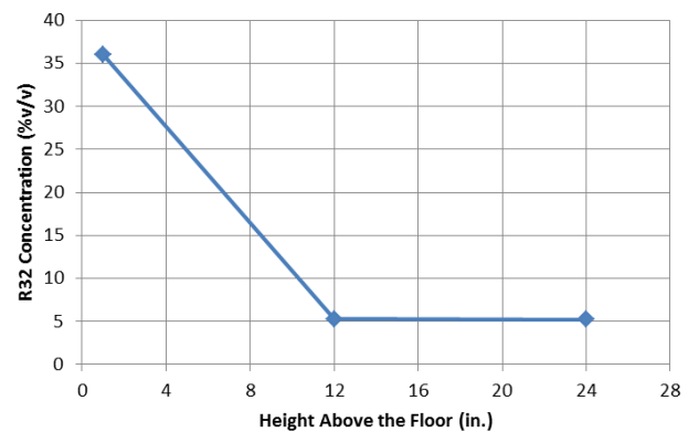
Refrigerant Concentration when Electric arcs are Energized
