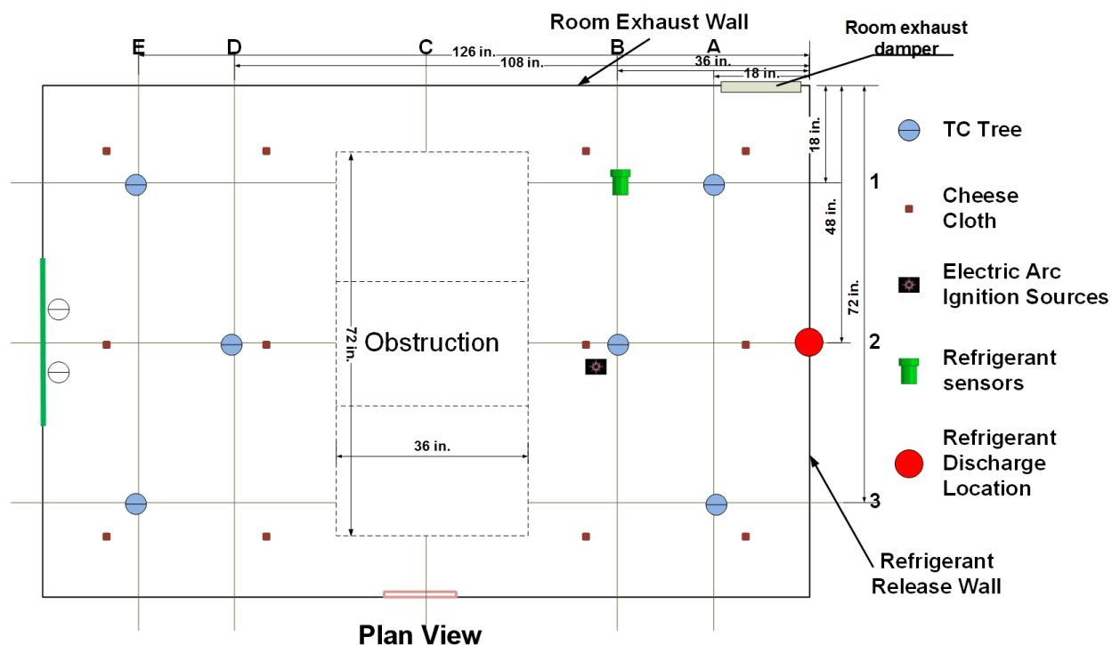
Figure 34 – Task 1 Instrumentation Plan
