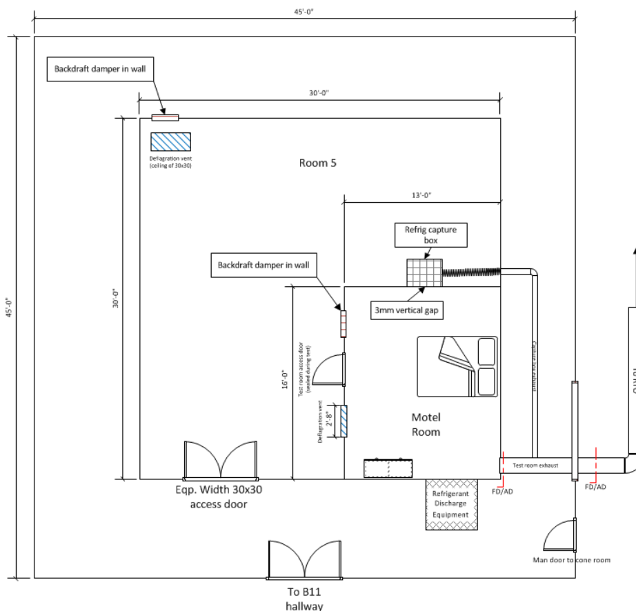
Figure 86 – Motel Room Layout within the 30'x30' test room
