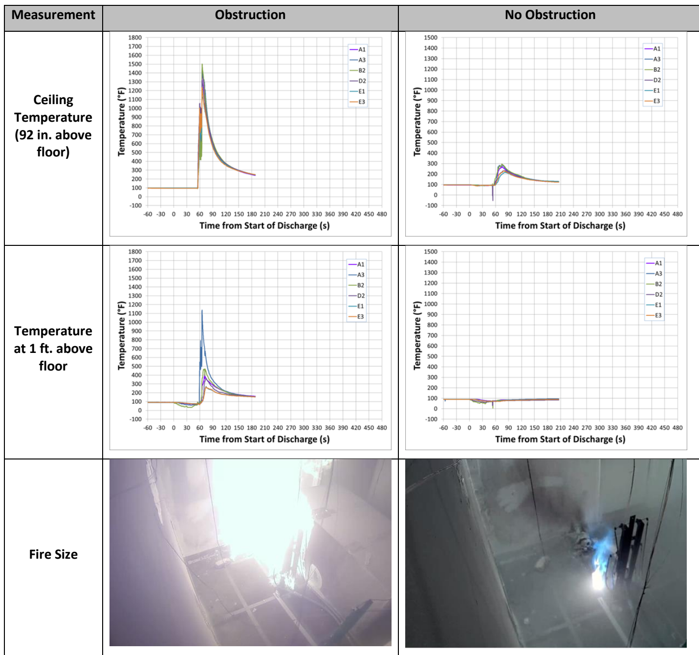
Figure 55 – Influence of Obstruction for R-452B Refrigerant
