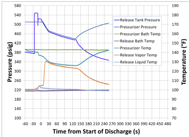
Pressure and Temperature in Pressurizer and Release Tanks
